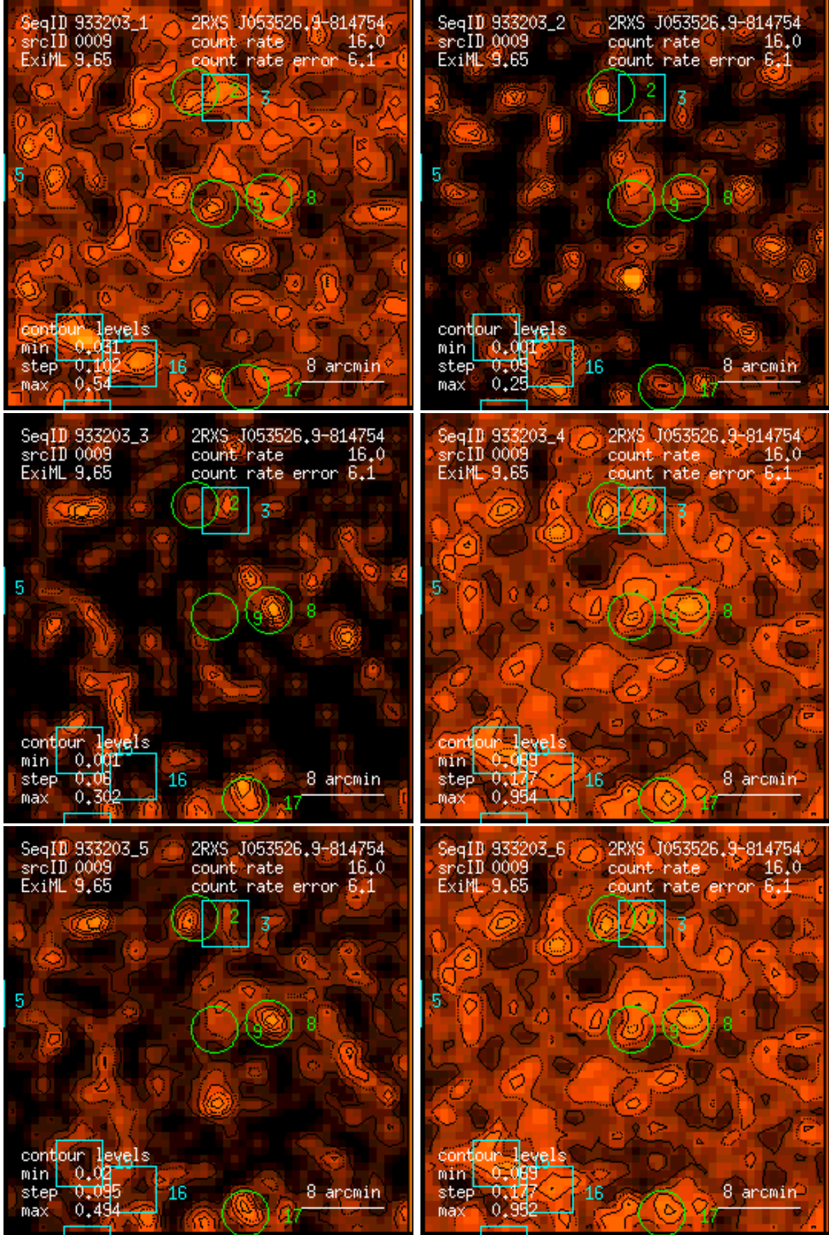
Figure 9: RASS 933203: detection 0009: band rate images, Gaussian filter: (1) PSPC channels 11 – 41, (2) 52 – 90, (3) 91 – 201, (4) 11 – 235, (5) 52 – 201, (6) 11 – 201. Broad band rates in counts/ks. Band rate contour levels in counts/ks/arcmin 2 .
