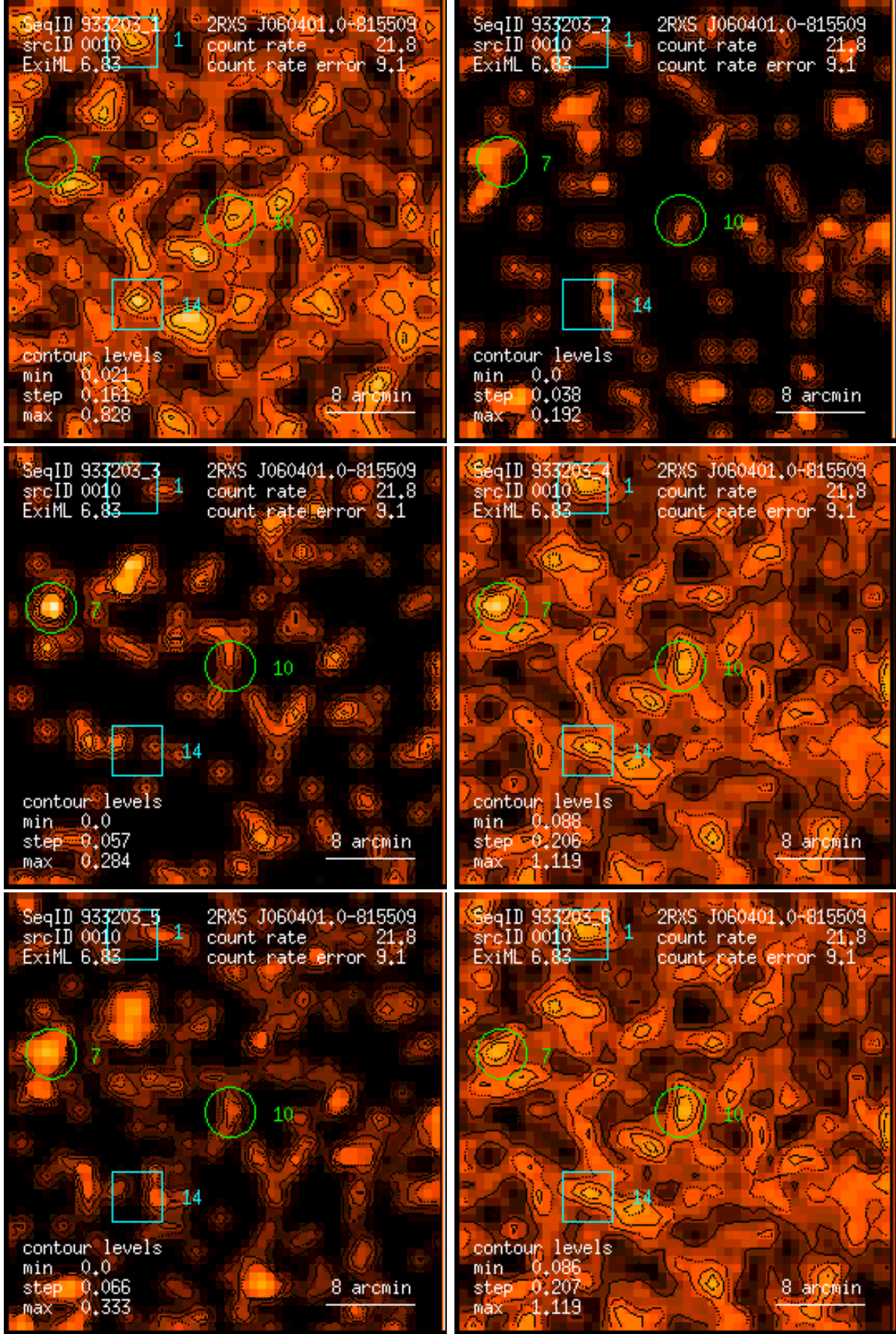
Figure 10: RASS 933203: detection 0010: band rate images, Gaussian filter: (1) PSPC channels 11 – 41, (2) 52 – 90, (3) 91 – 201, (4) 11 – 235, (5) 52 – 201, (6) 11 – 201. Broad band rates in counts/ks. Band rate contour levels in counts/ks/arcmin 2 .
