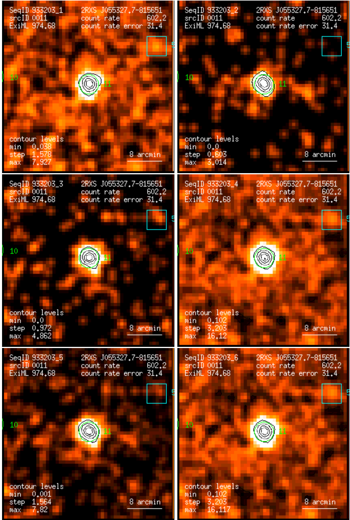
Figure 11: RASS 933203: detection 0011: band rate images, Gaussian filter: (1) PSPC channels 11 – 41, (2) 52 – 90, (3) 91 – 201, (4) 11 – 235, (5) 52 – 201, (6) 11 – 201. Broad band rates in counts/ks. Band rate contour levels in counts/ks/arcmin 2 .
