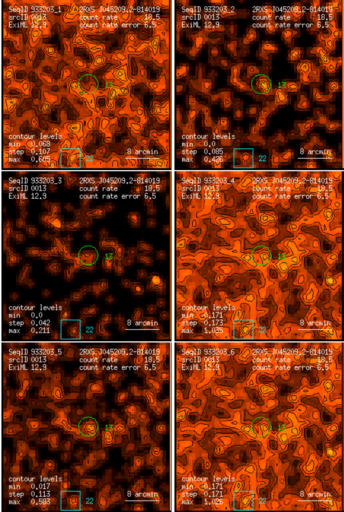
Figure 13: RASS 933203: detection 0013: band rate images, Gaussian filter: (1) PSPC channels 11 – 41, (2) 52 – 90, (3) 91 – 201, (4) 11 – 235, (5) 52 – 201, (6) 11 – 201. Broad band rates in counts/ks. Band rate contour levels in counts/ks/arcmin 2 .
