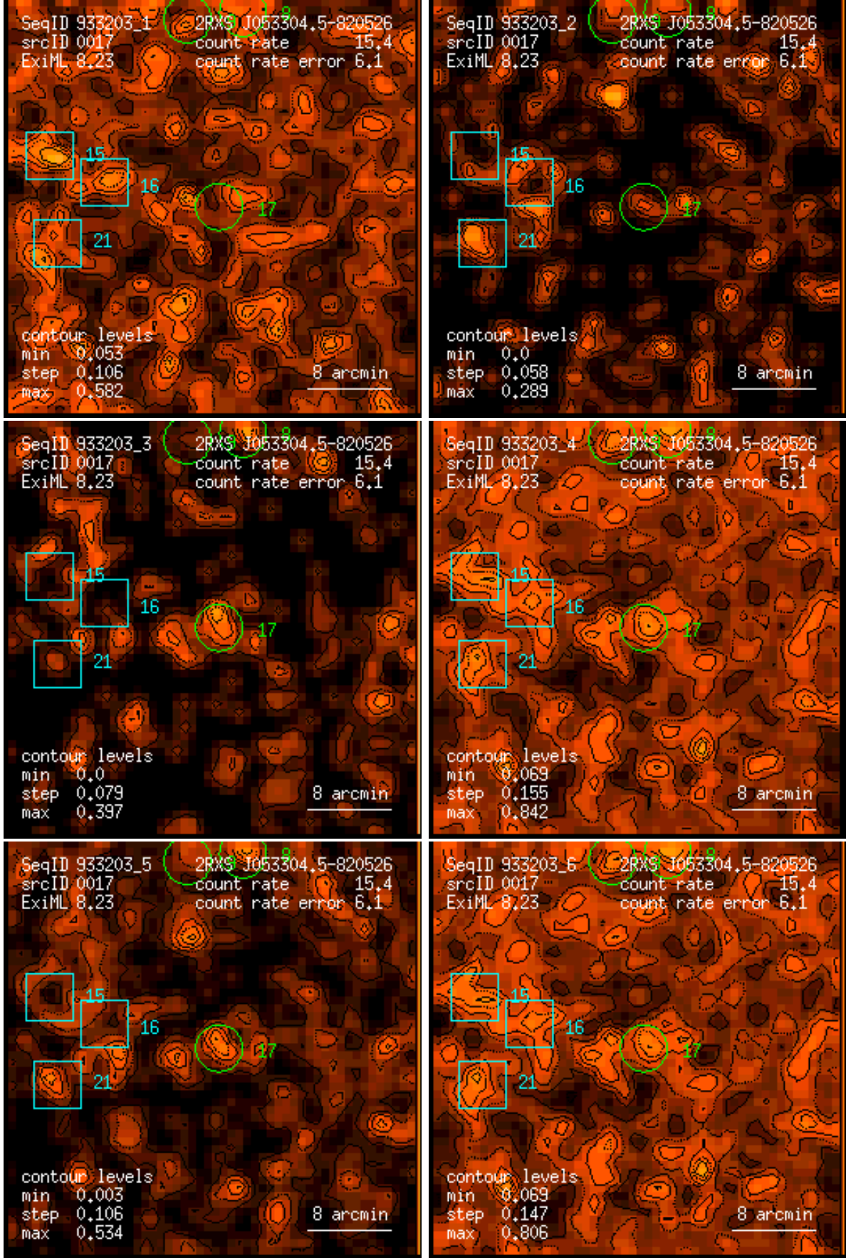
Figure 17: RASS 933203: detection 0017: band rate images, Gaussian filter: (1) PSPC channels 11 – 41, (2) 52 – 90, (3) 91 – 201, (4) 11 – 235, (5) 52 – 201, (6) 11 – 201. Broad band rates in counts/ks. Band rate contour levels in counts/ks/arcmin 2 .
