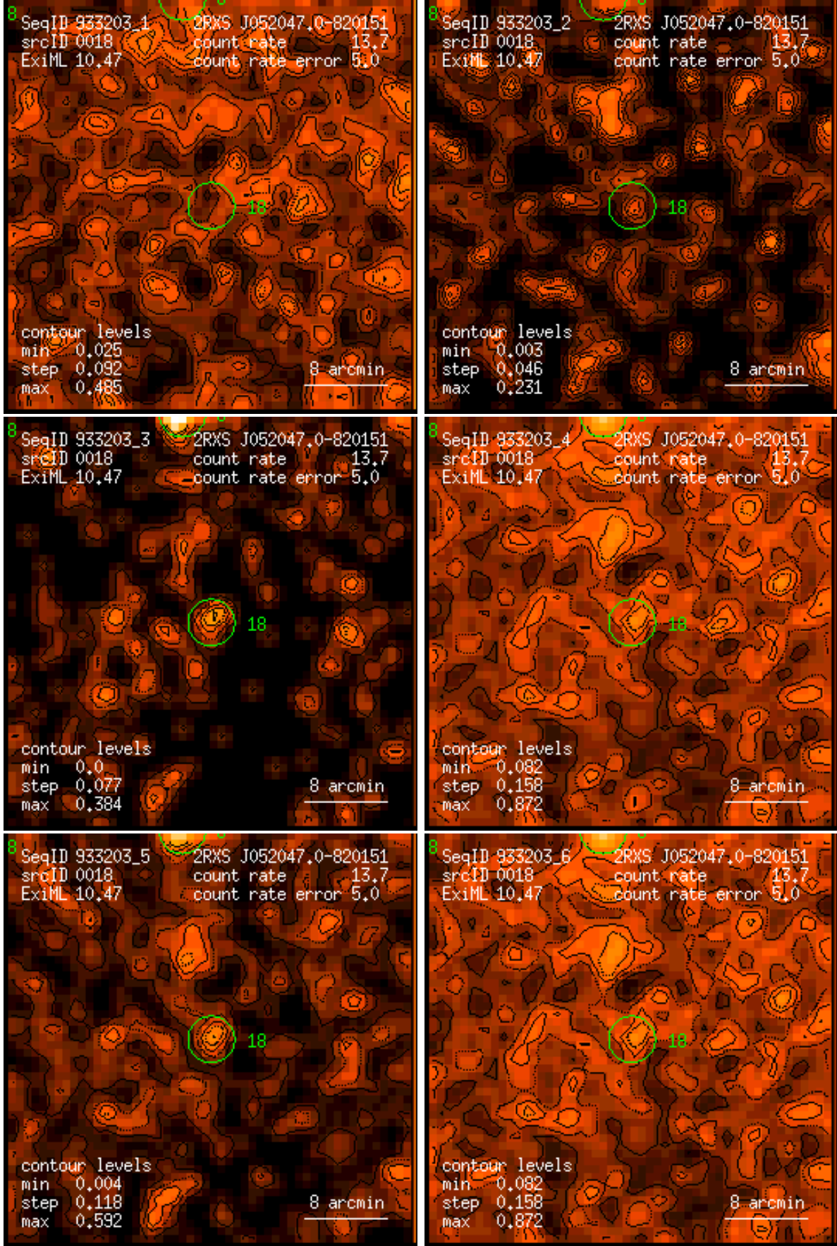
Figure 18: RASS 933203: detection 0018: band rate images, Gaussian filter: (1) PSPC channels 11 – 41, (2) 52 – 90, (3) 91 – 201, (4) 11 – 235, (5) 52 – 201, (6) 11 – 201. Broad band rates in counts/ks. Band rate contour levels in counts/ks/arcmin 2 .
