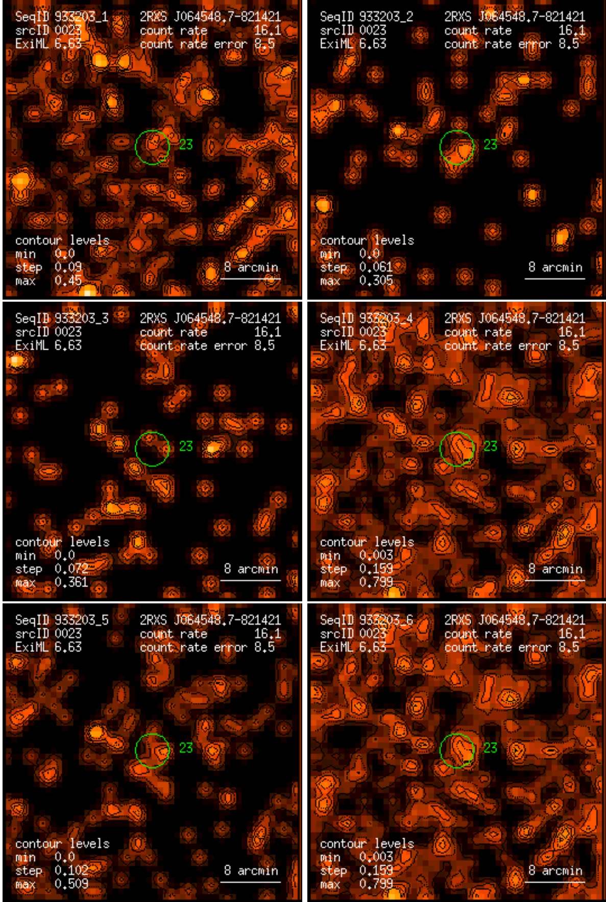
Figure 23: RASS 933203: detection 0023: band rate images, Gaussian filter: (1) PSPC channels 11 – 41, (2) 52 – 90, (3) 91 – 201, (4) 11 – 235, (5) 52 – 201, (6) 11 – 201. Broad band rates in counts/ks. Band rate contour levels in counts/ks/arcmin 2 .
