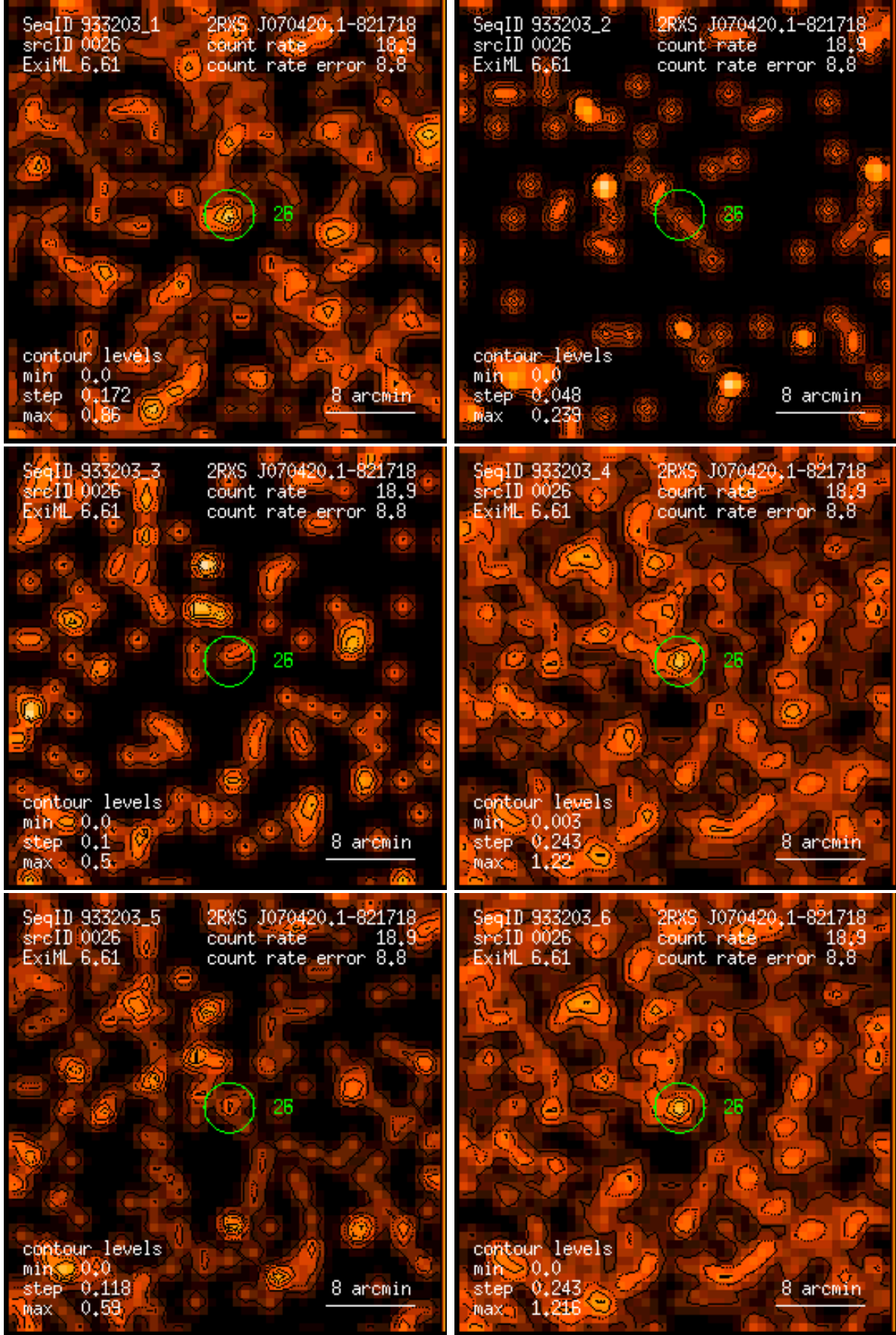
Figure 26: RASS 933203: detection 0026: band rate images, Gaussian filter: (1) PSPC channels 11 – 41, (2) 52 – 90, (3) 91 – 201, (4) 11 – 235, (5) 52 – 201, (6) 11 – 201. Broad band rates in counts/ks. Band rate contour levels in counts/ks/arcmin 2 .
