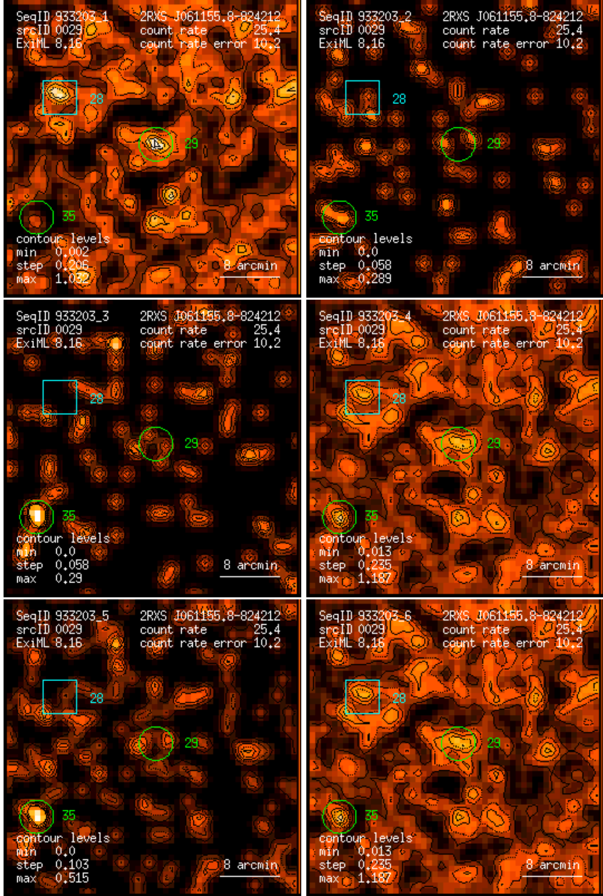
Figure 29: RASS 933203: detection 0029: band rate images, Gaussian filter: (1) PSPC channels 11 – 41, (2) 52 – 90, (3) 91 – 201, (4) 11 – 235, (5) 52 – 201, (6) 11 – 201. Broad band rates in counts/ks. Band rate contour levels in counts/ks/arcmin 2 .
