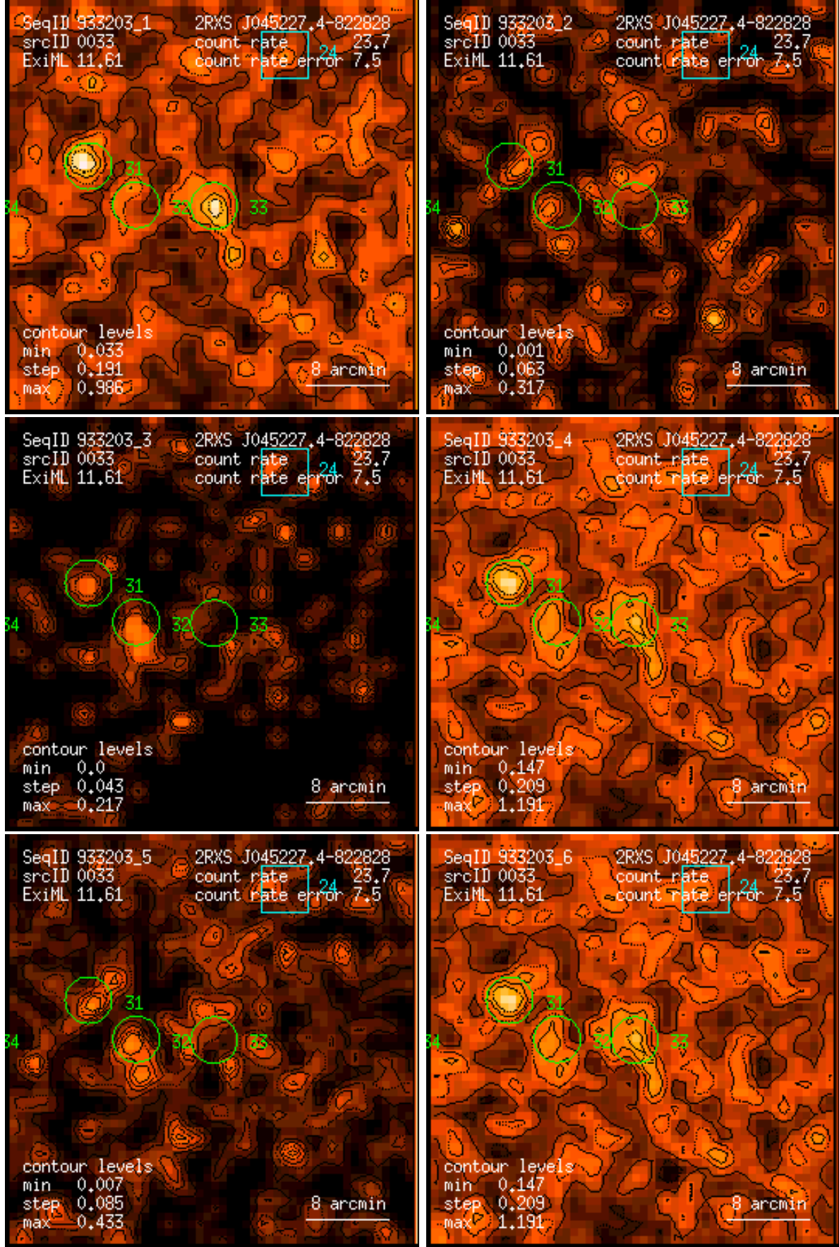
Figure 33: RASS 933203: detection 0033: band rate images, Gaussian filter: (1) PSPC channels 11 – 41, (2) 52 – 90, (3) 91 – 201, (4) 11 – 235, (5) 52 – 201, (6) 11 – 201. Broad band rates in counts/ks. Band rate contour levels in counts/ks/arcmin 2 .
