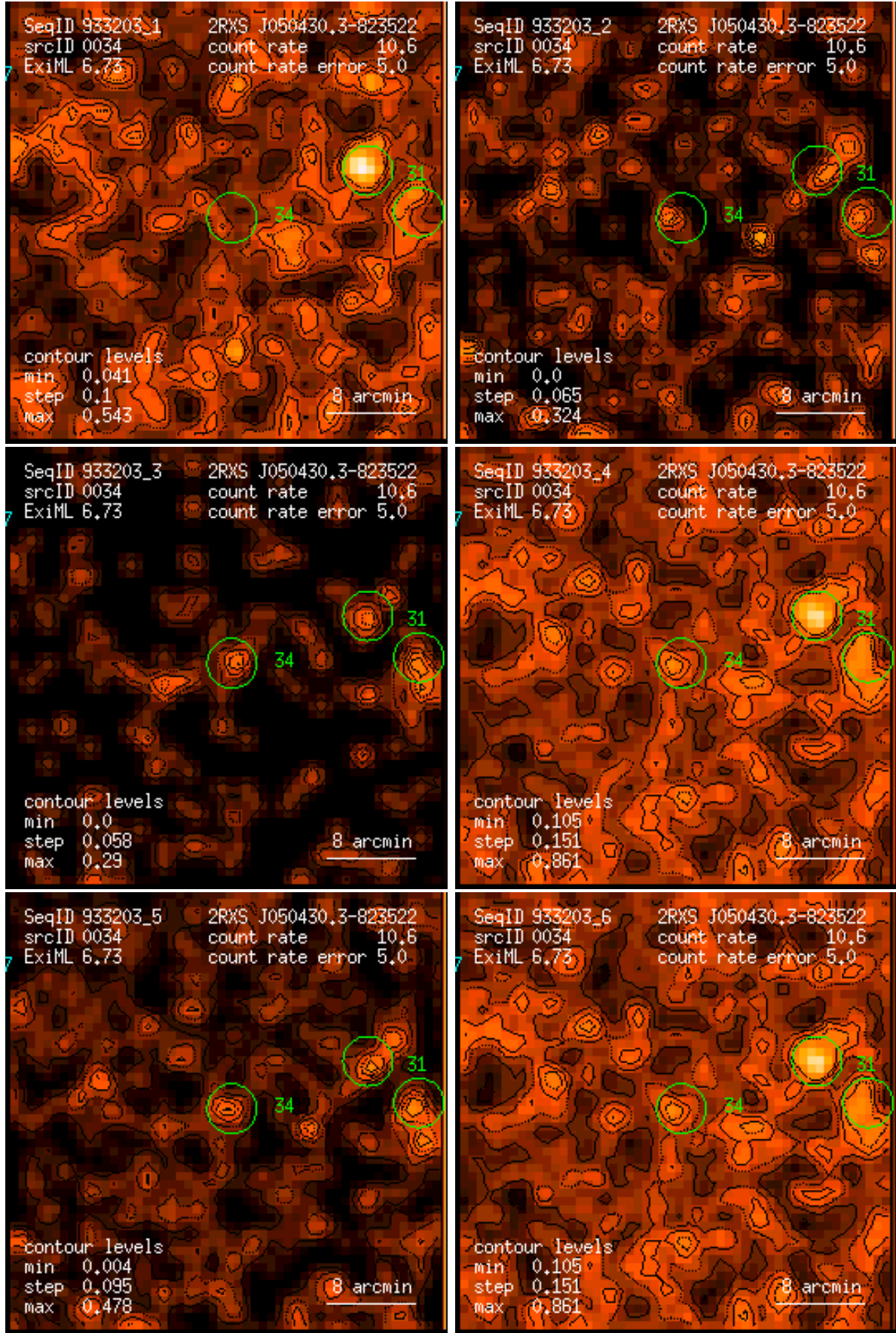
Figure 34: RASS 933203: detection 0034: band rate images, Gaussian filter: (1) PSPC channels 11 – 41, (2) 52 – 90, (3) 91 – 201, (4) 11 – 235, (5) 52 – 201, (6) 11 – 201. Broad band rates in counts/ks. Band rate contour levels in counts/ks/arcmin 2 .
