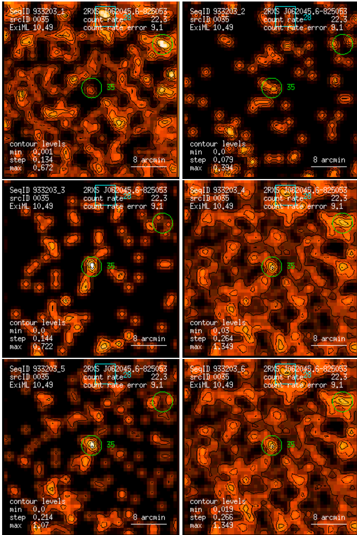
Figure 35: RASS 933203: detection 0035: band rate images, Gaussian filter: (1) PSPC channels 11 – 41, (2) 52 – 90, (3) 91 – 201, (4) 11 – 235, (5) 52 – 201, (6) 11 – 201. Broad band rates in counts/ks. Band rate contour levels in counts/ks/arcmin 2 .
