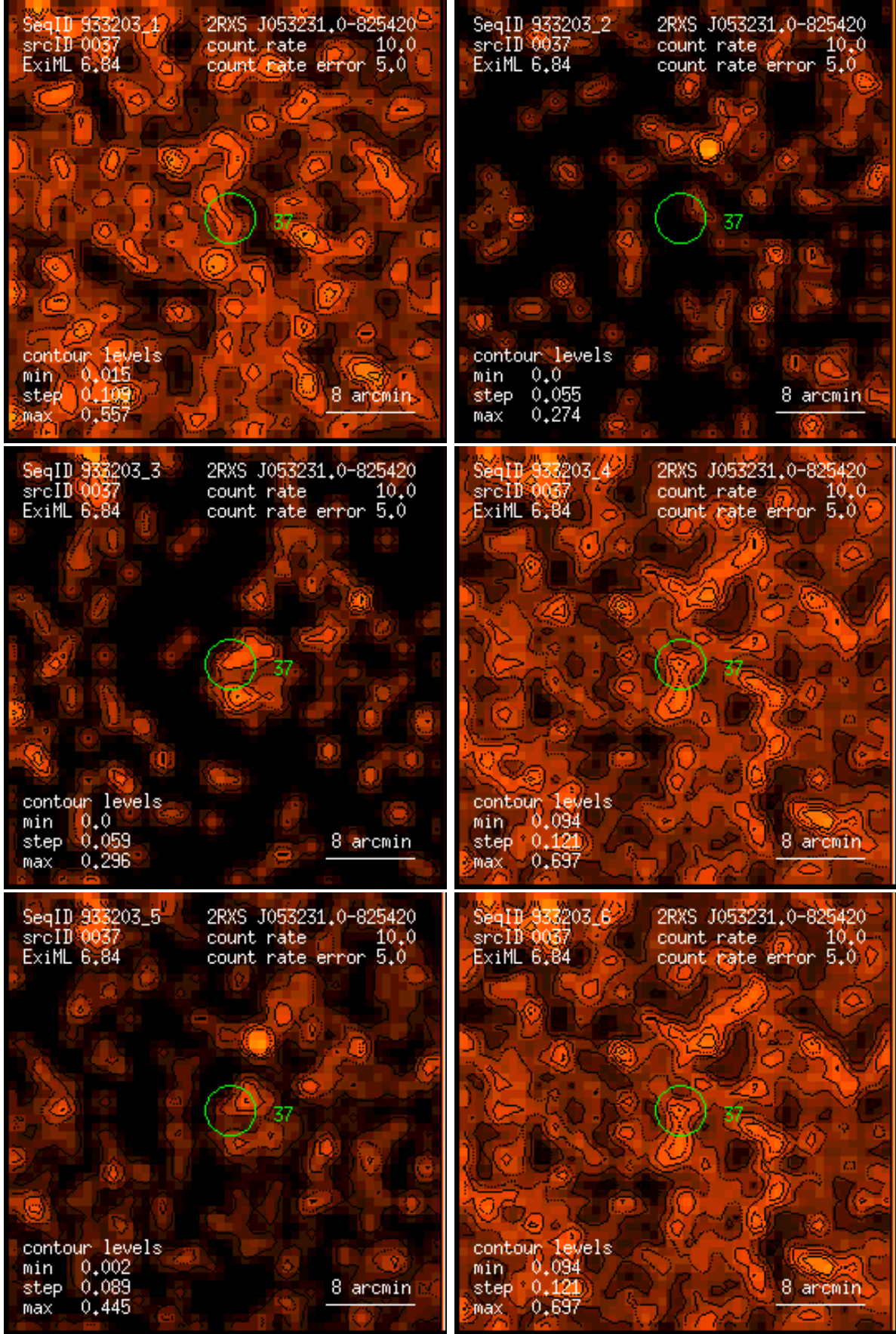
Figure 37: RASS 933203: detection 0037: band rate images, Gaussian filter: (1) PSPC channels 11 – 41, (2) 52 – 90, (3) 91 – 201, (4) 11 – 235, (5) 52 – 201, (6) 11 – 201. Broad band rates in counts/ks. Band rate contour levels in counts/ks/arcmin 2 .
