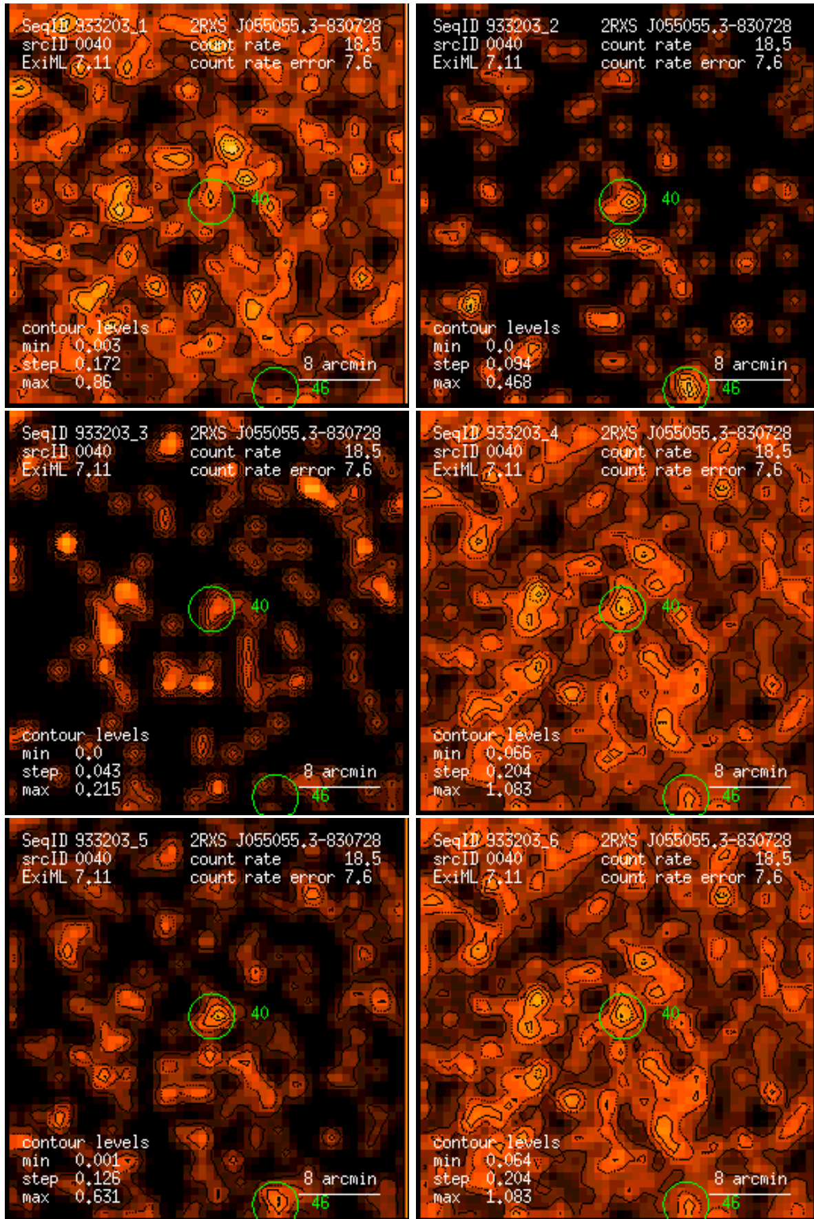
Figure 40: RASS 933203: detection 0040: band rate images, Gaussian filter: (1) PSPC channels 11 – 41, (2) 52 – 90, (3) 91 – 201, (4) 11 – 235, (5) 52 – 201, (6) 11 – 201. Broad band rates in counts/ks. Band rate contour levels in counts/ks/arcmin 2 .
