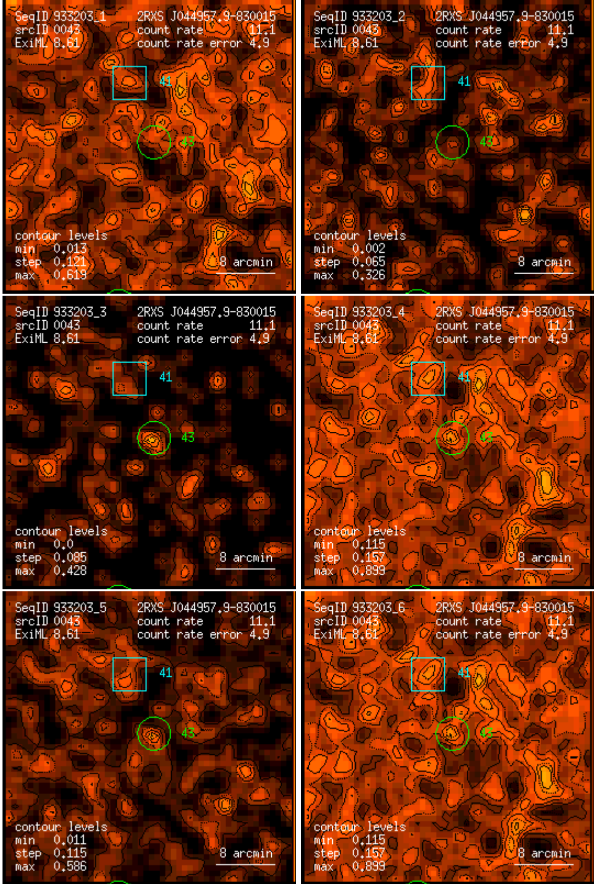
Figure 43: RASS 933203: detection 0043: band rate images, Gaussian filter: (1) PSPC channels 11 – 41, (2) 52 – 90, (3) 91 – 201, (4) 11 – 235, (5) 52 – 201, (6) 11 – 201. Broad band rates in counts/ks. Band rate contour levels in counts/ks/arcmin 2 .
