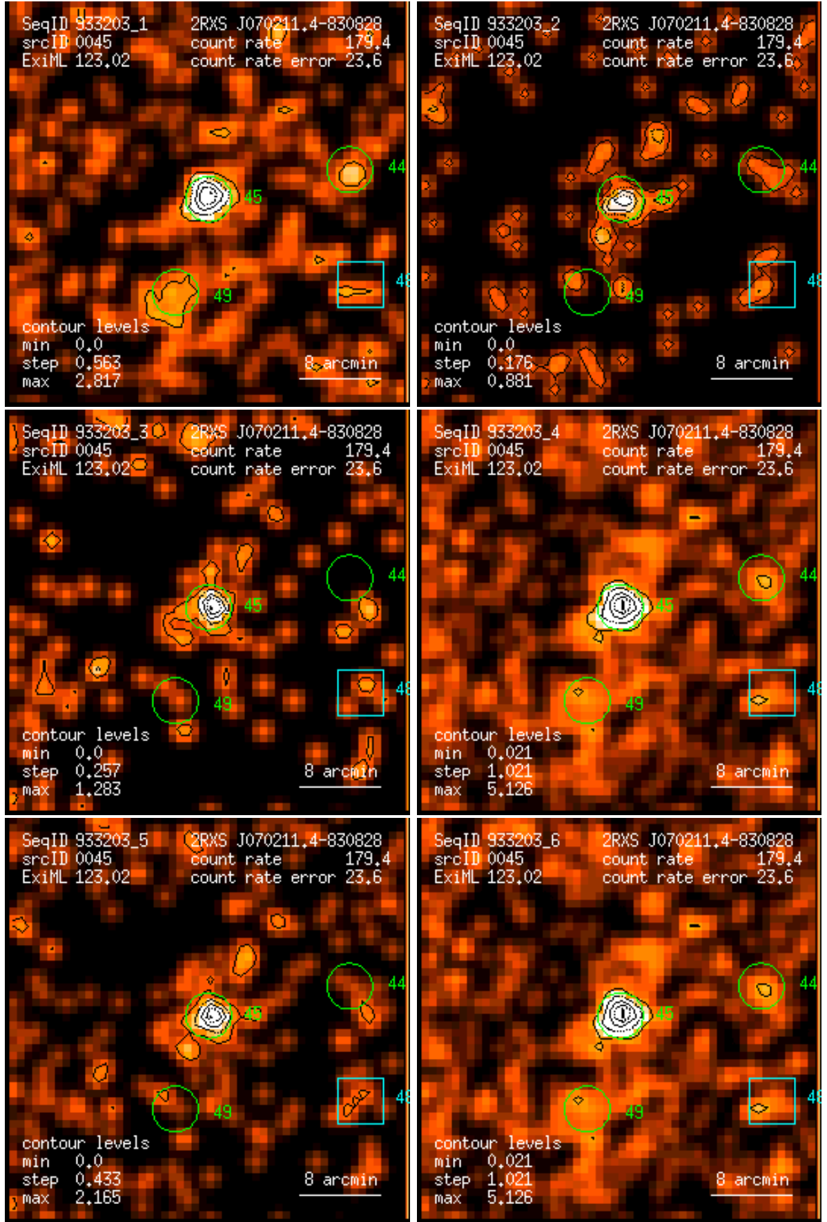
Figure 45: RASS 933203: detection 0045: band rate images, Gaussian filter: (1) PSPC channels 11 – 41, (2) 52 – 90, (3) 91 – 201, (4) 11 – 235, (5) 52 – 201, (6) 11 – 201. Broad band rates in counts/ks. Band rate contour levels in counts/ks/arcmin 2 .
