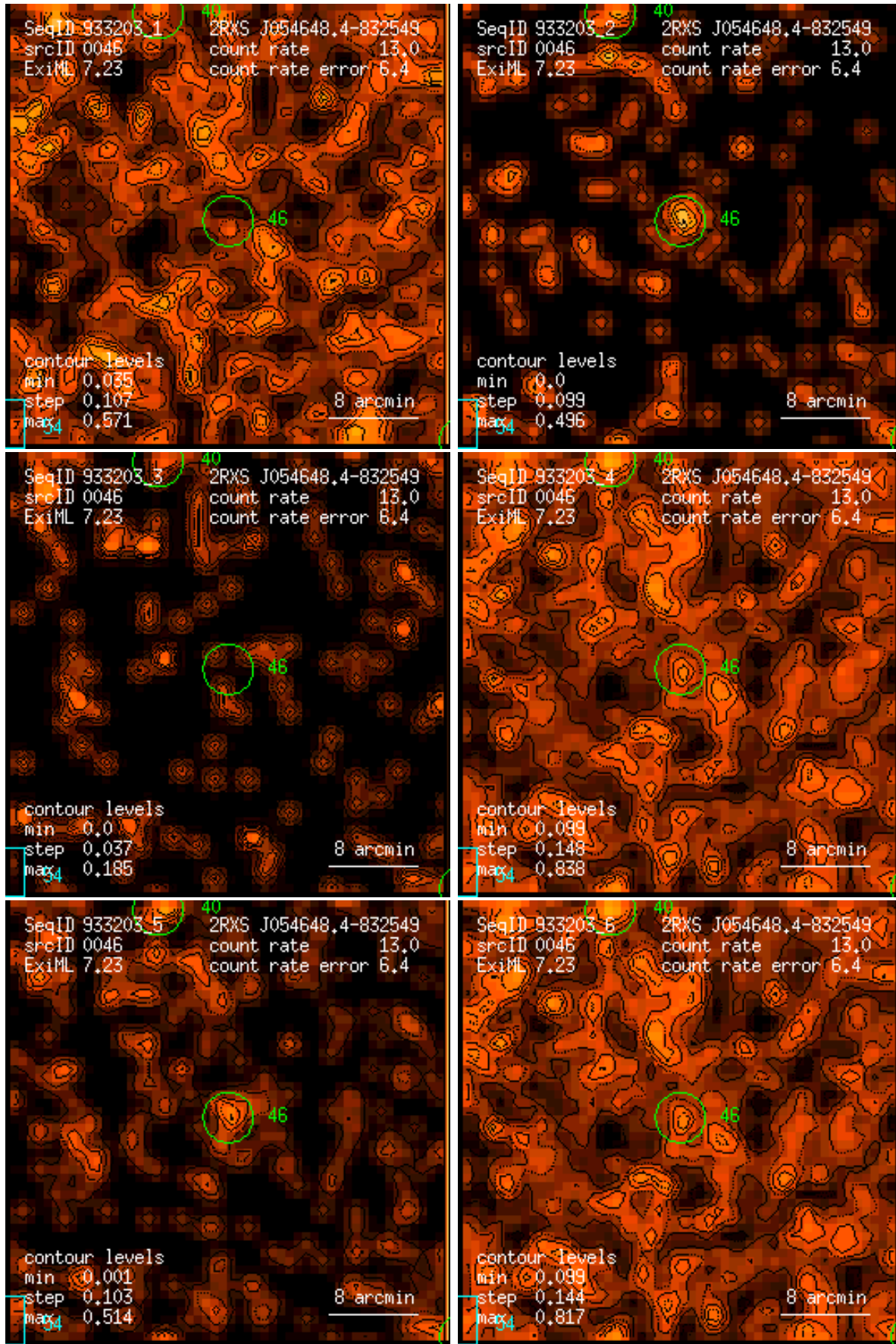
Figure 46: RASS 933203: detection 0046: band rate images, Gaussian filter: (1) PSPC channels 11 – 41, (2) 52 – 90, (3) 91 – 201, (4) 11 – 235, (5) 52 – 201, (6) 11 – 201. Broad band rates in counts/ks. Band rate contour levels in counts/ks/arcmin 2 .
