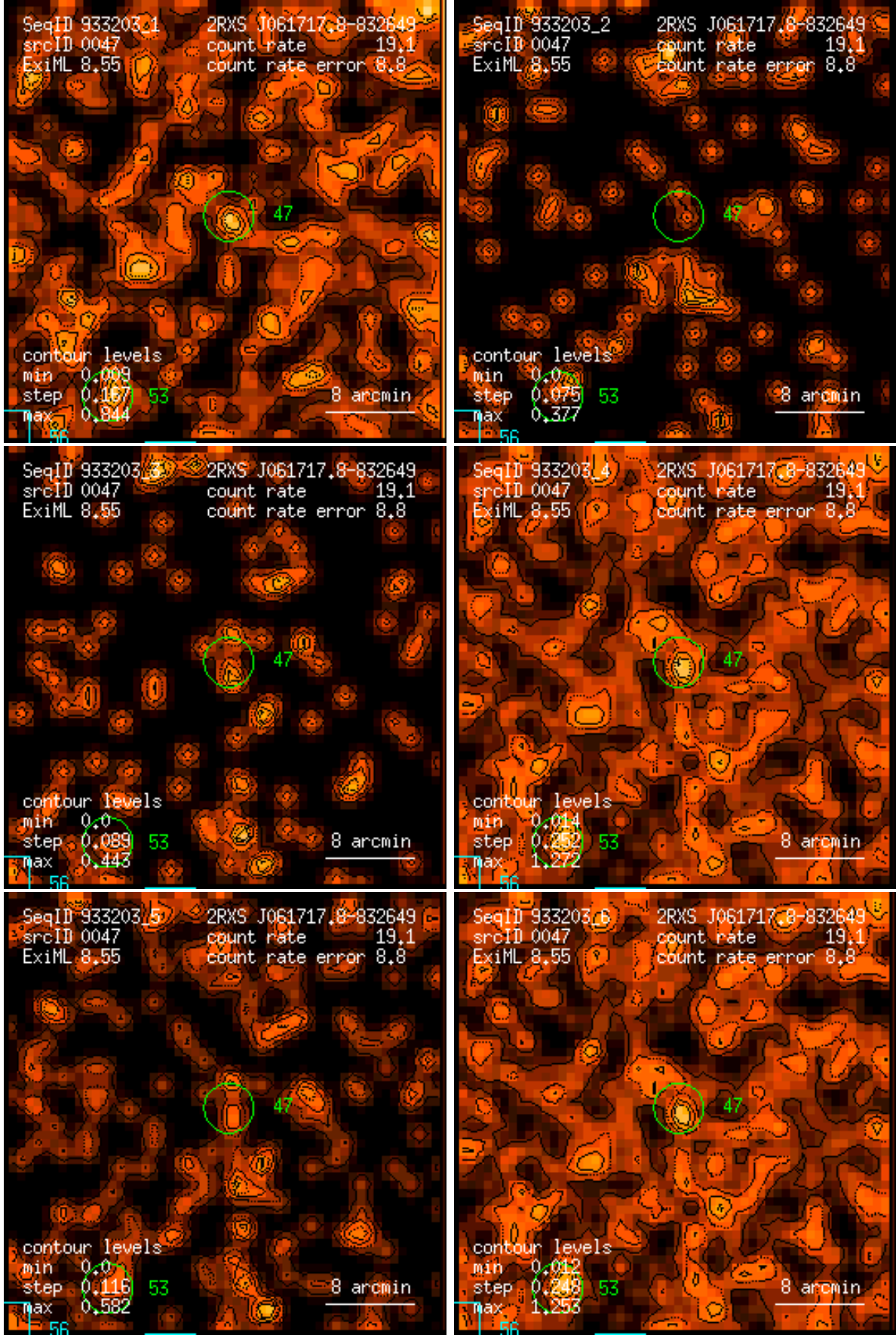
Figure 47: RASS 933203: detection 0047: band rate images, Gaussian filter: (1) PSPC channels 11 – 41, (2) 52 – 90, (3) 91 – 201, (4) 11 – 235, (5) 52 – 201, (6) 11 – 201. Broad band rates in counts/ks. Band rate contour levels in counts/ks/arcmin 2 .
