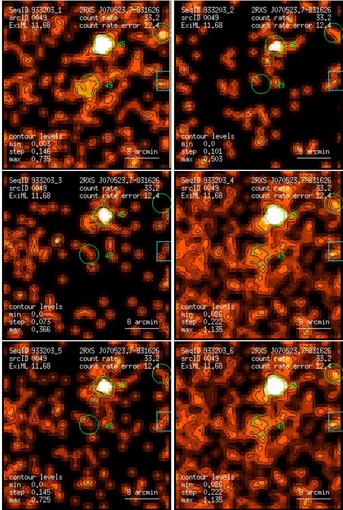
Figure 49: RASS 933203: detection 0049: band rate images, Gaussian filter: (1) PSPC channels 11 – 41, (2) 52 – 90, (3) 91 – 201, (4) 11 – 235, (5) 52 – 201, (6) 11 – 201. Broad band rates in counts/ks. Band rate contour levels in counts/ks/arcmin 2 .
