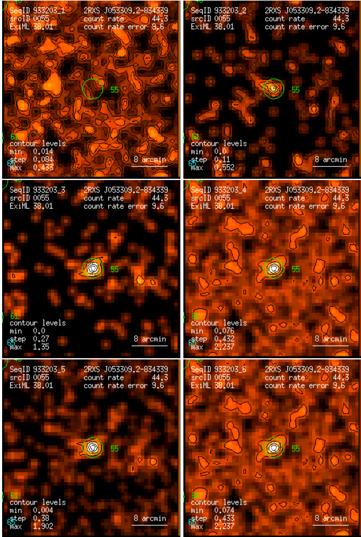
Figure 55: RASS 933203: detection 0055: band rate images, Gaussian filter: (1) PSPC channels 11 – 41, (2) 52 – 90, (3) 91 – 201, (4) 11 – 235, (5) 52 – 201, (6) 11 – 201. Broad band rates in counts/ks. Band rate contour levels in counts/ks/arcmin 2 .
