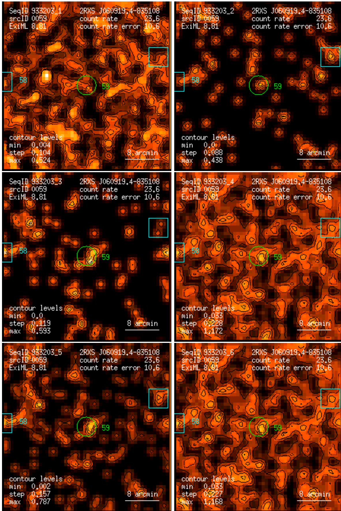
Figure 59: RASS 933203: detection 0059: band rate images, Gaussian filter: (1) PSPC channels 11 – 41, (2) 52 – 90, (3) 91 – 201, (4) 11 – 235, (5) 52 – 201, (6) 11 – 201. Broad band rates in counts/ks. Band rate contour levels in counts/ks/arcmin 2 .
