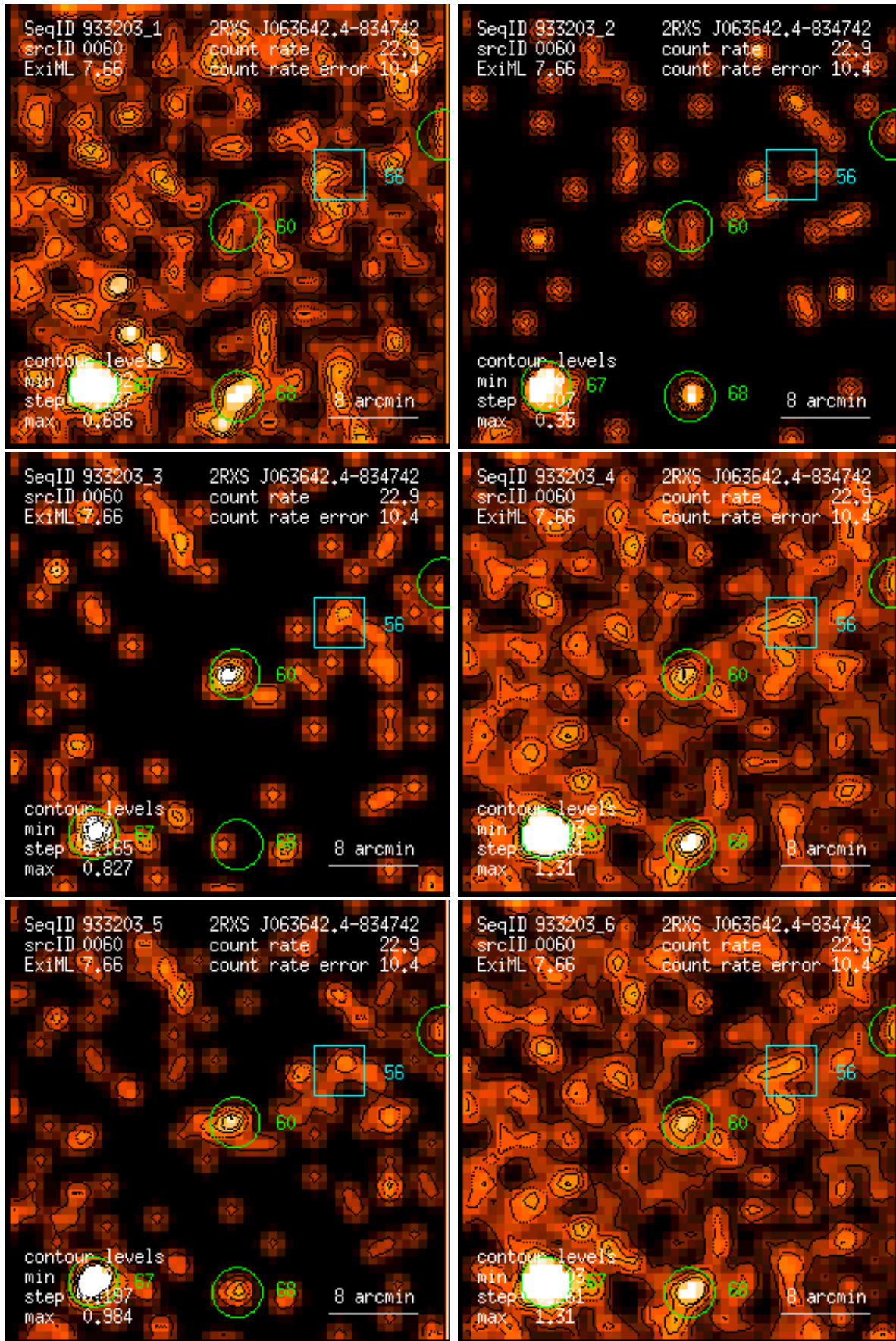
Figure 60: RASS 933203: detection 0060: band rate images, Gaussian filter: (1) PSPC channels 11 – 41, (2) 52 – 90, (3) 91 – 201, (4) 11 – 235, (5) 52 – 201, (6) 11 – 201. Broad band rates in counts/ks. Band rate contour levels in counts/ks/arcmin 2 .
