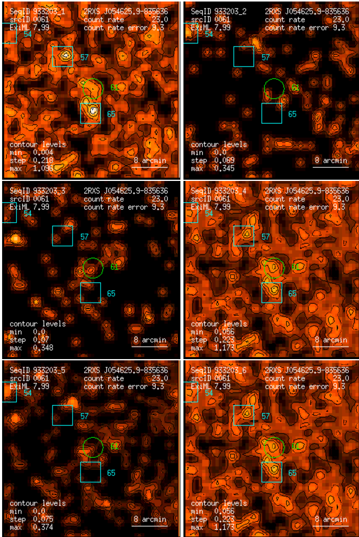
Figure 61: RASS 933203: detection 0061: band rate images, Gaussian filter: (1) PSPC channels 11 – 41, (2) 52 – 90, (3) 91 – 201, (4) 11 – 235, (5) 52 – 201, (6) 11 – 201. Broad band rates in counts/ks. Band rate contour levels in counts/ks/arcmin 2 .
