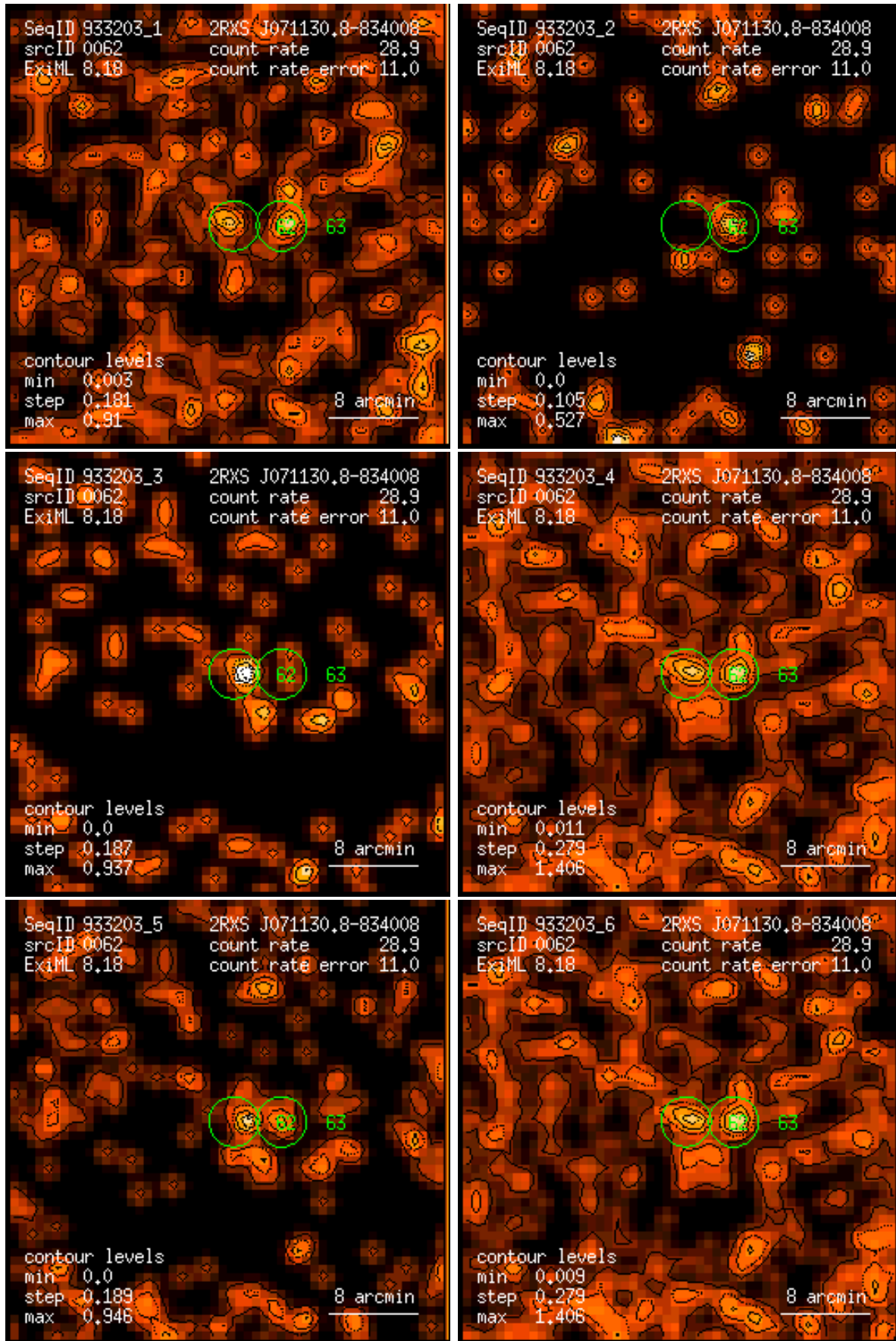
Figure 62: RASS 933203: detection 0062: band rate images, Gaussian filter: (1) PSPC channels 11 – 41, (2) 52 – 90, (3) 91 – 201, (4) 11 – 235, (5) 52 – 201, (6) 11 – 201. Broad band rates in counts/ks. Band rate contour levels in counts/ks/arcmin 2 .
