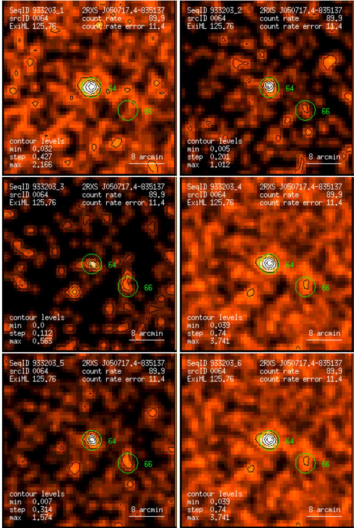
Figure 64: RASS 933203: detection 0064: band rate images, Gaussian filter: (1) PSPC channels 11 – 41, (2) 52 – 90, (3) 91 – 201, (4) 11 – 235, (5) 52 – 201, (6) 11 – 201. Broad band rates in counts/ks. Band rate contour levels in counts/ks/arcmin 2 .
