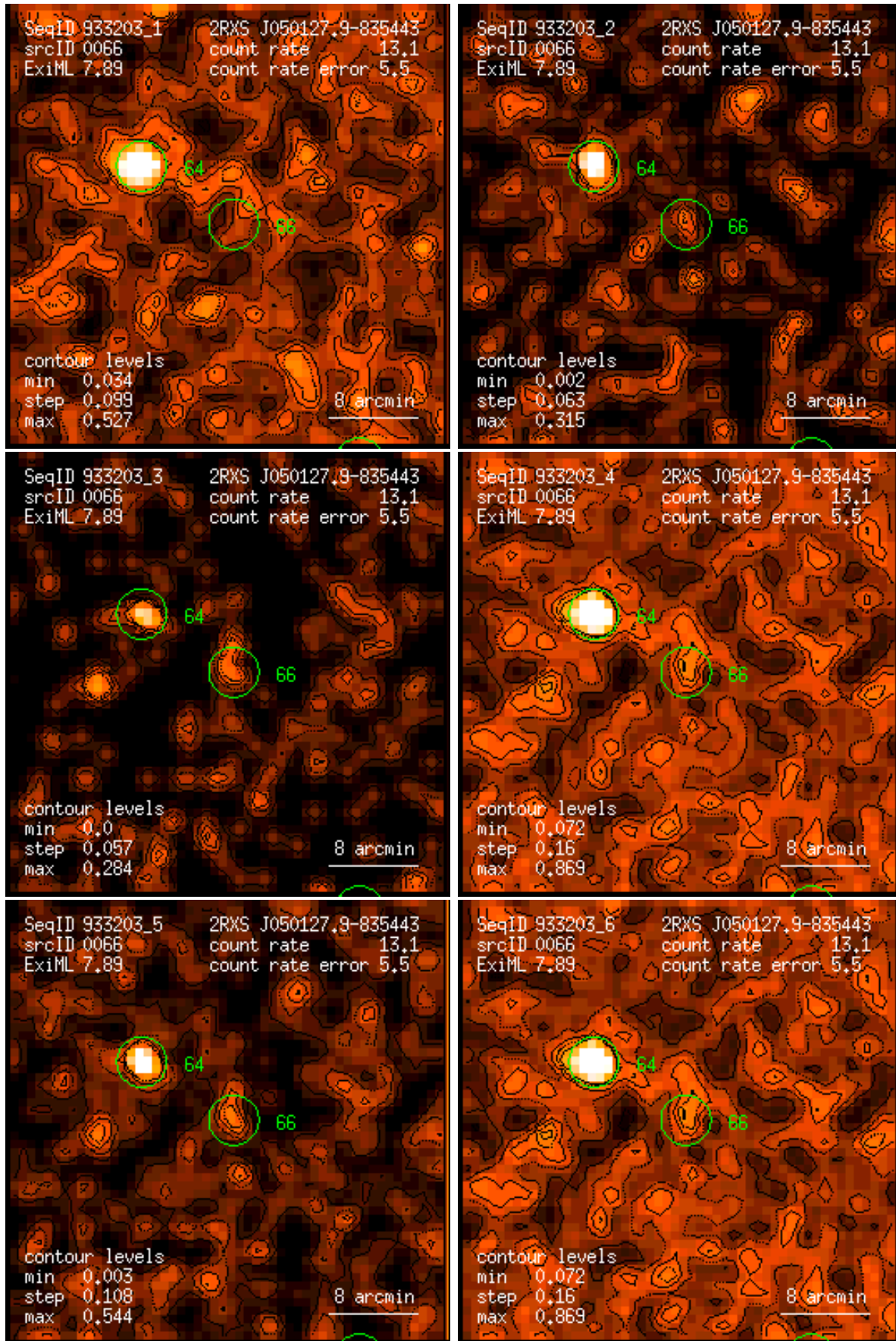
Figure 66: RASS 933203: detection 0066: band rate images, Gaussian filter: (1) PSPC channels 11 – 41, (2) 52 – 90, (3) 91 – 201, (4) 11 – 235, (5) 52 – 201, (6) 11 – 201. Broad band rates in counts/ks. Band rate contour levels in counts/ks/arcmin 2 .
