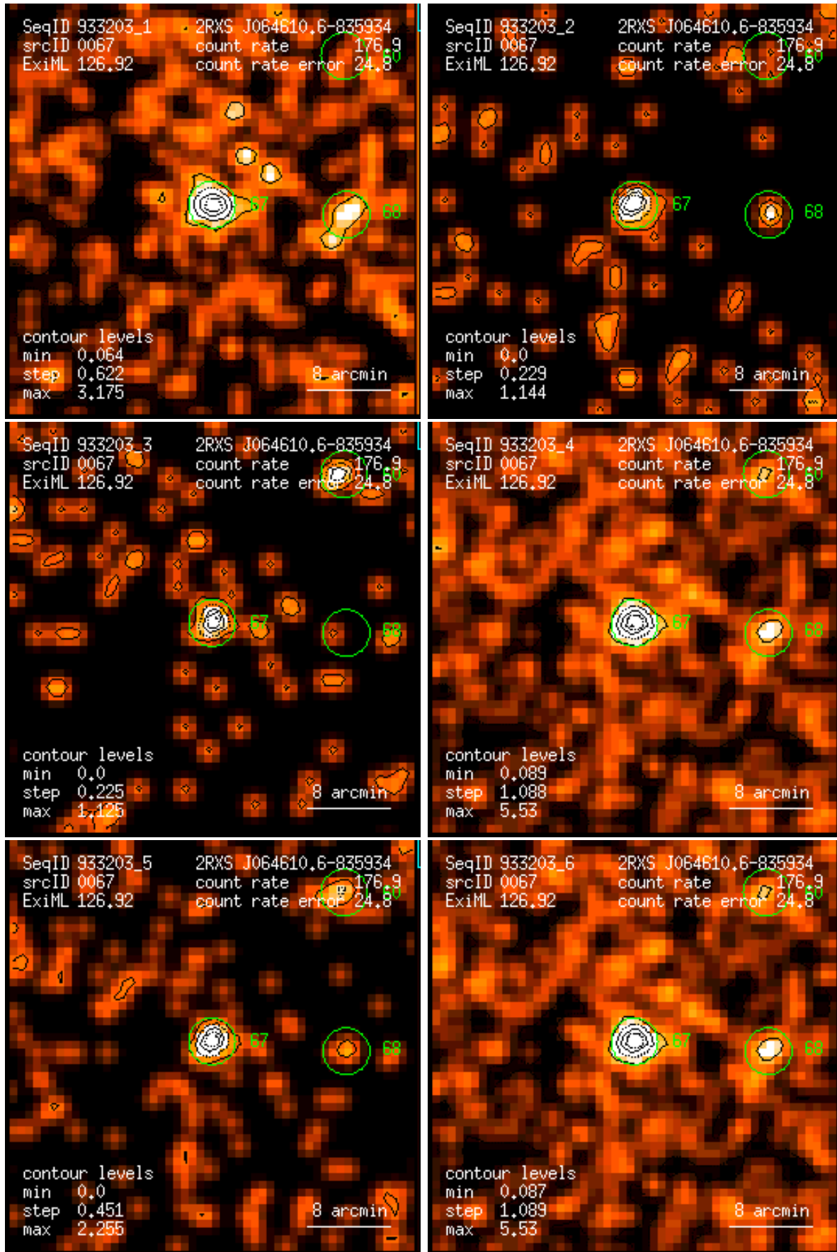
Figure 67: RASS 933203: detection 0067: band rate images, Gaussian filter: (1) PSPC channels 11 – 41, (2) 52 – 90, (3) 91 – 201, (4) 11 – 235, (5) 52 – 201, (6) 11 – 201. Broad band rates in counts/ks. Band rate contour levels in counts/ks/arcmin 2 .
