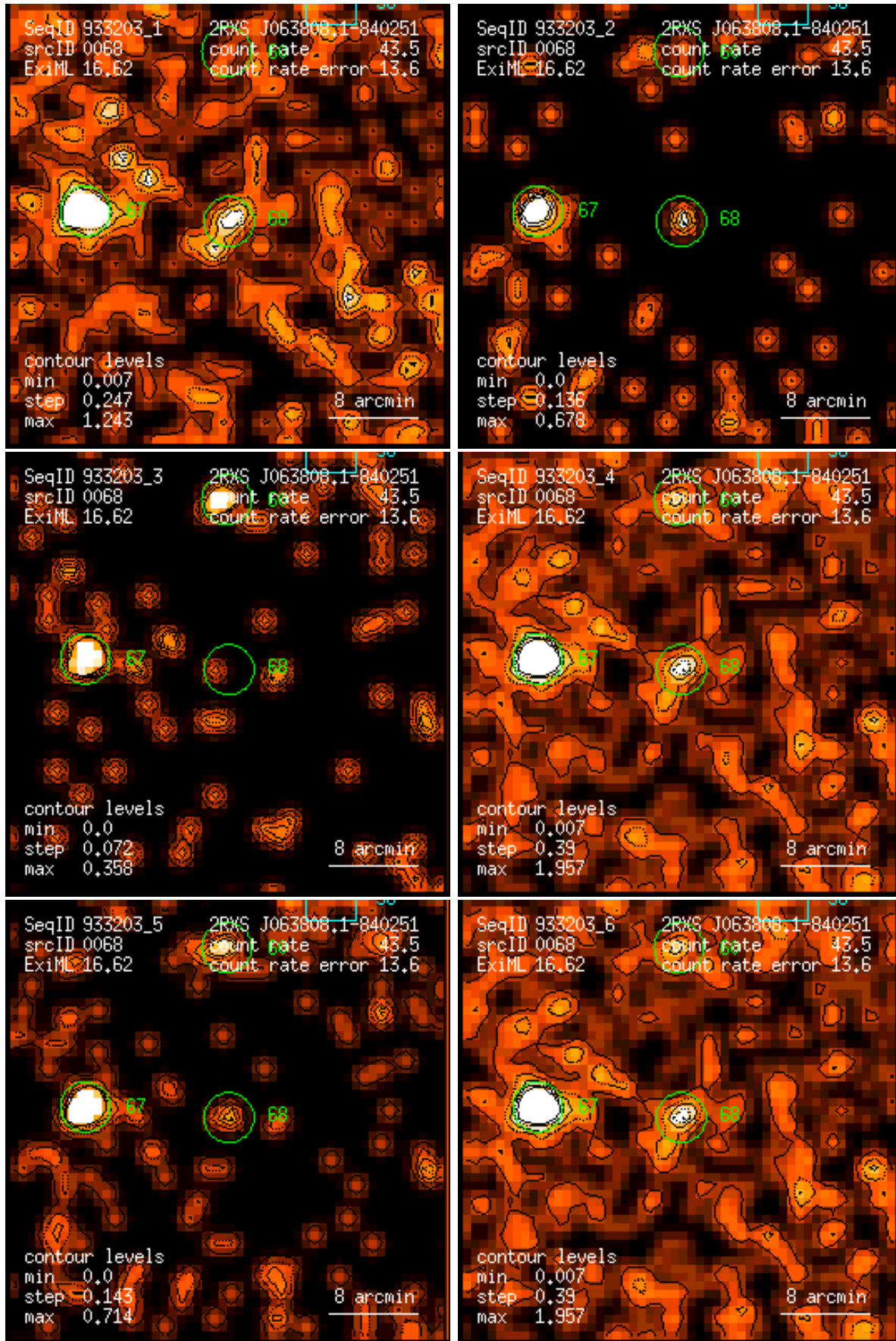
Figure 68: RASS 933203: detection 0068: band rate images, Gaussian filter: (1) PSPC channels 11 – 41, (2) 52 – 90, (3) 91 – 201, (4) 11 – 235, (5) 52 – 201, (6) 11 – 201. Broad band rates in counts/ks. Band rate contour levels in counts/ks/arcmin 2 .
