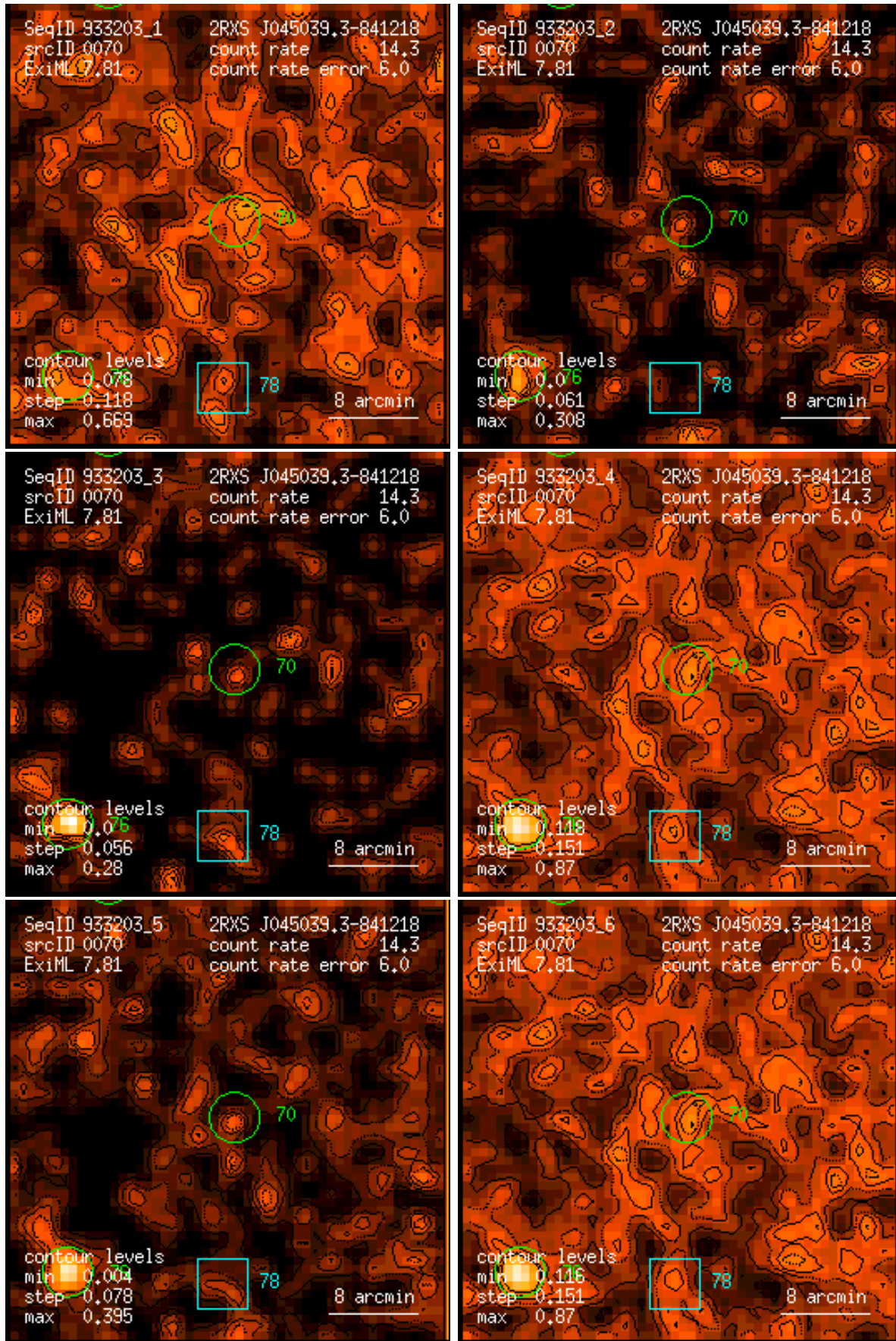
Figure 70: RASS 933203: detection 0070: band rate images, Gaussian filter: (1) PSPC channels 11 – 41, (2) 52 – 90, (3) 91 – 201, (4) 11 – 235, (5) 52 – 201, (6) 11 – 201. Broad band rates in counts/ks. Band rate contour levels in counts/ks/arcmin 2 .
