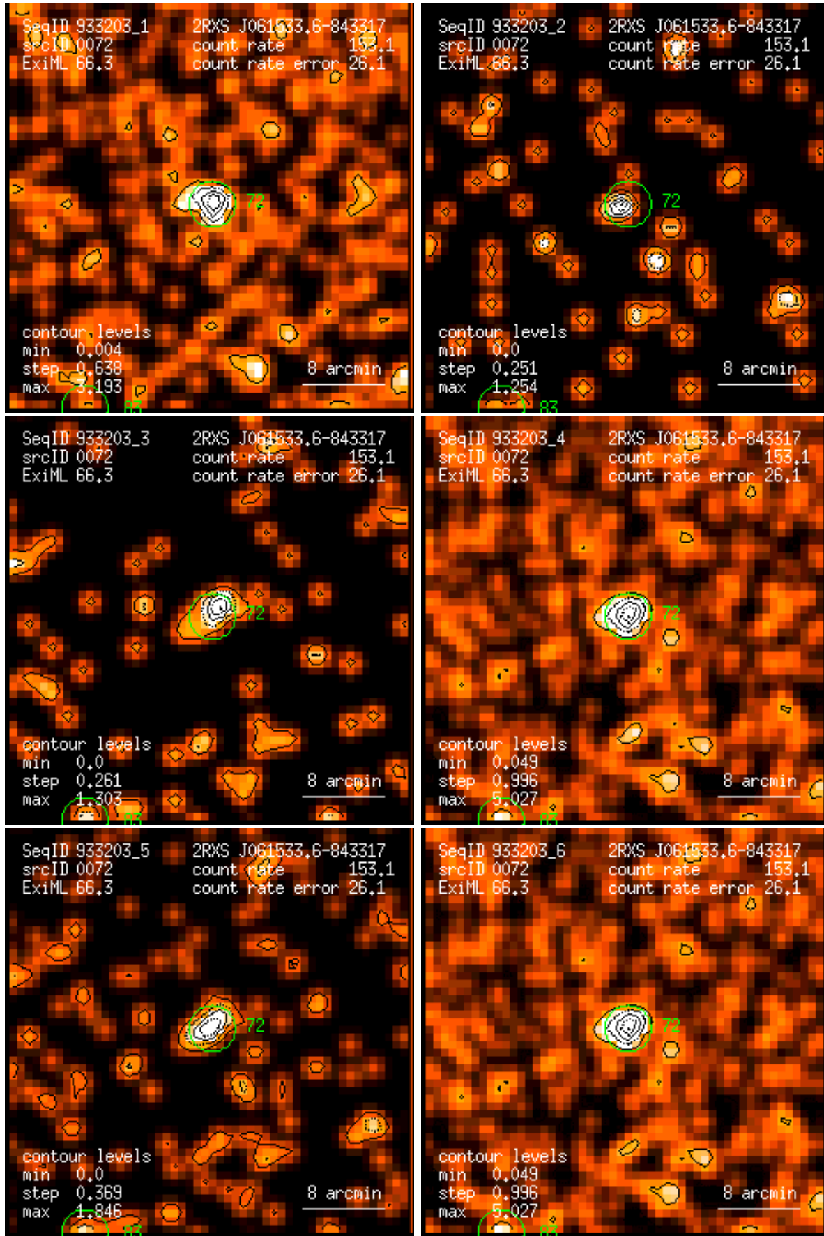
Figure 72: RASS 933203: detection 0072: band rate images, Gaussian filter: (1) PSPC channels 11 – 41, (2) 52 – 90, (3) 91 – 201, (4) 11 – 235, (5) 52 – 201, (6) 11 – 201. Broad band rates in counts/ks. Band rate contour levels in counts/ks/arcmin 2 .
