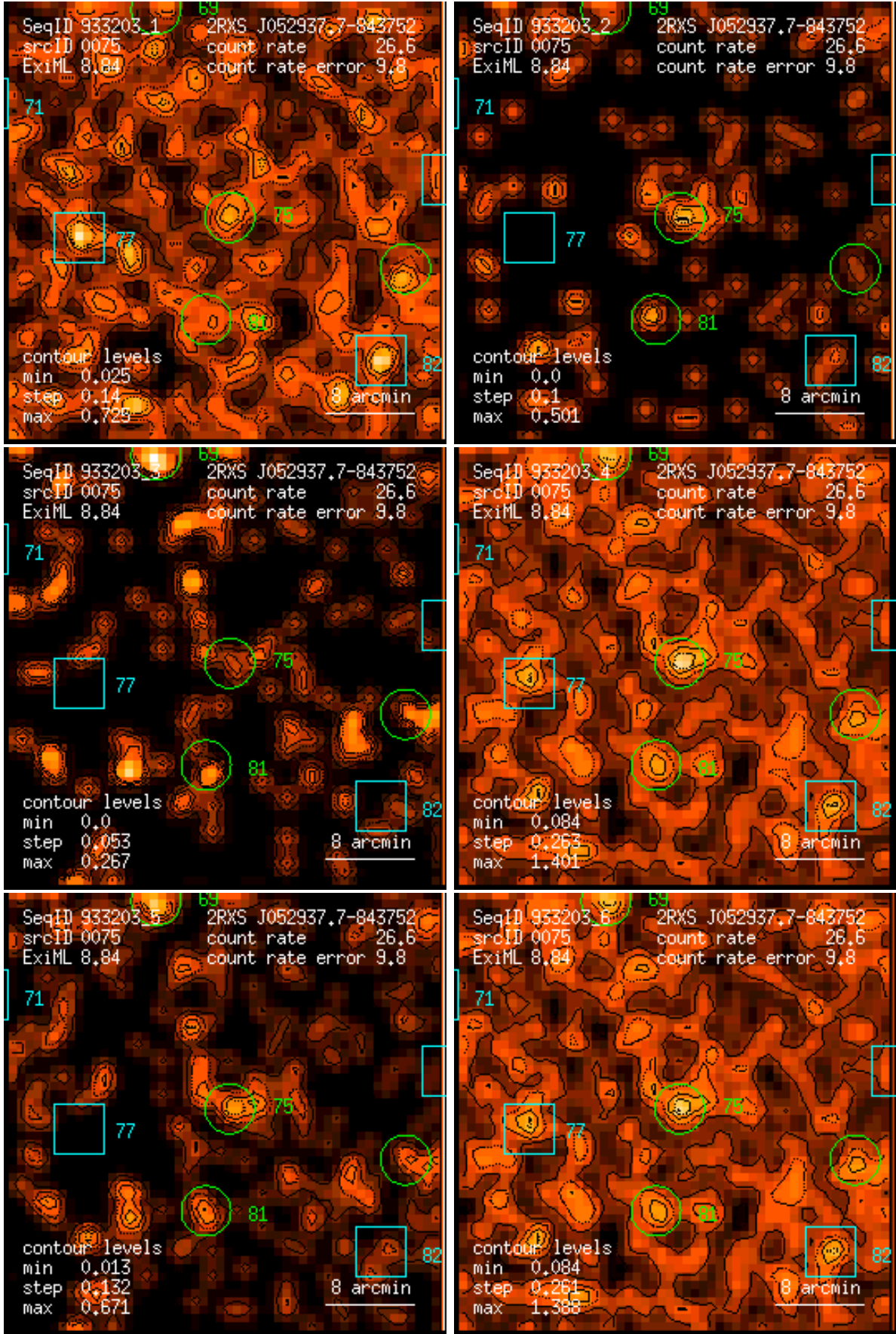
Figure 75: RASS 933203: detection 0075: band rate images, Gaussian filter: (1) PSPC channels 11 – 41, (2) 52 – 90, (3) 91 – 201, (4) 11 – 235, (5) 52 – 201, (6) 11 – 201. Broad band rates in counts/ks. Band rate contour levels in counts/ks/arcmin 2 .
