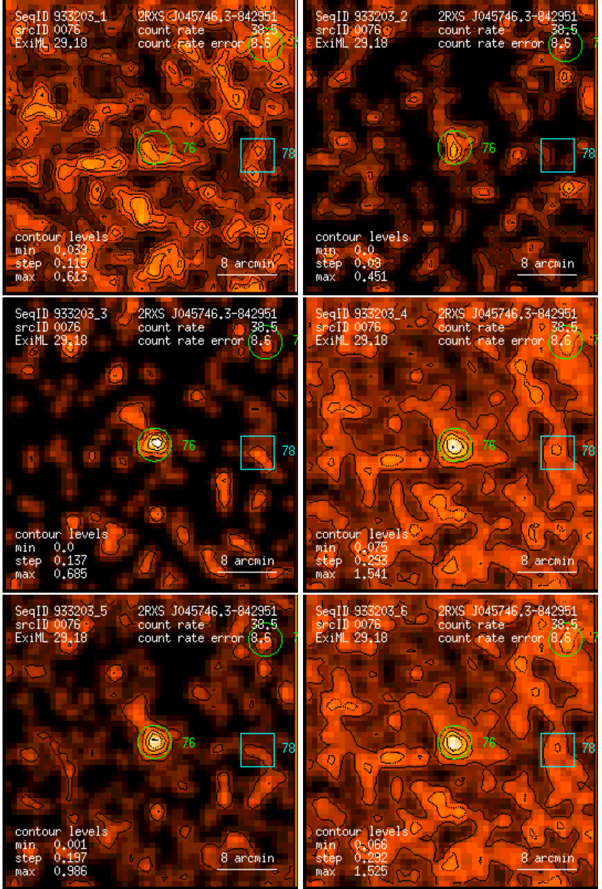
Figure 76: RASS 933203: detection 0076: band rate images, Gaussian filter: (1) PSPC channels 11 – 41, (2) 52 – 90, (3) 91 – 201, (4) 11 – 235, (5) 52 – 201, (6) 11 – 201. Broad band rates in counts/ks. Band rate contour levels in counts/ks/arcmin 2 .
