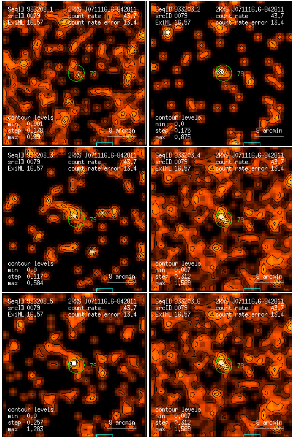
Figure 79: RASS 933203: detection 0079: band rate images, Gaussian filter: (1) PSPC channels 11 – 41, (2) 52 – 90, (3) 91 – 201, (4) 11 – 235, (5) 52 – 201, (6) 11 – 201. Broad band rates in counts/ks. Band rate contour levels in counts/ks/arcmin 2 .
