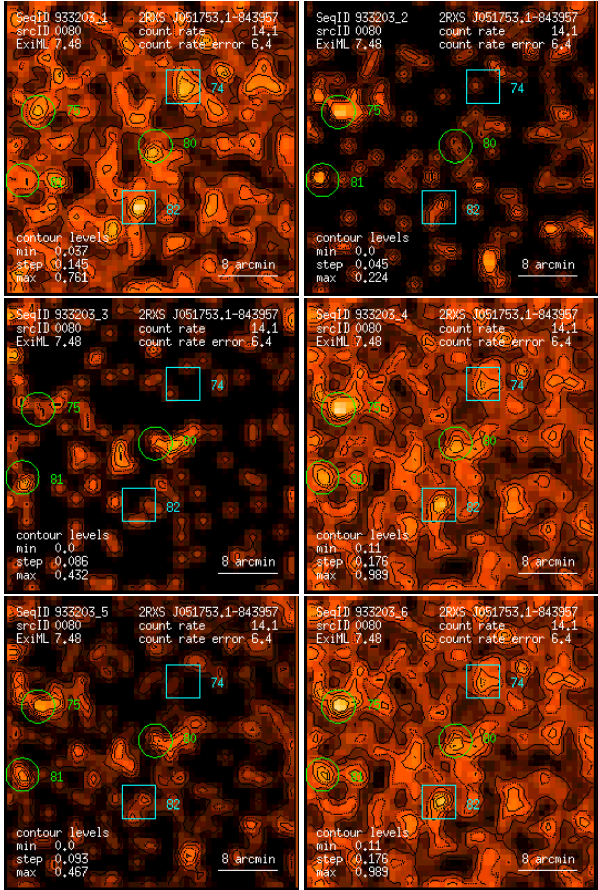
Figure 80: RASS 933203: detection 0080: band rate images, Gaussian filter: (1) PSPC channels 11 – 41, (2) 52 – 90, (3) 91 – 201, (4) 11 – 235, (5) 52 – 201, (6) 11 – 201. Broad band rates in counts/ks. Band rate contour levels in counts/ks/arcmin 2 .
