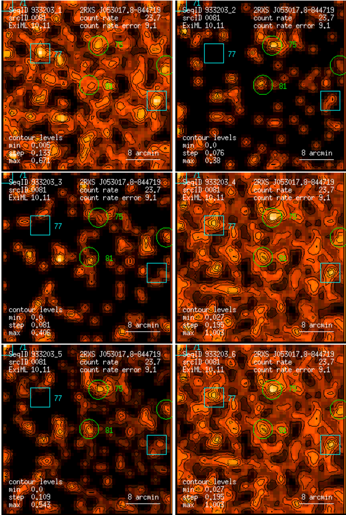
Figure 81: RASS 933203: detection 0081: band rate images, Gaussian filter: (1) PSPC channels 11 – 41, (2) 52 – 90, (3) 91 – 201, (4) 11 – 235, (5) 52 – 201, (6) 11 – 201. Broad band rates in counts/ks. Band rate contour levels in counts/ks/arcmin 2 .
