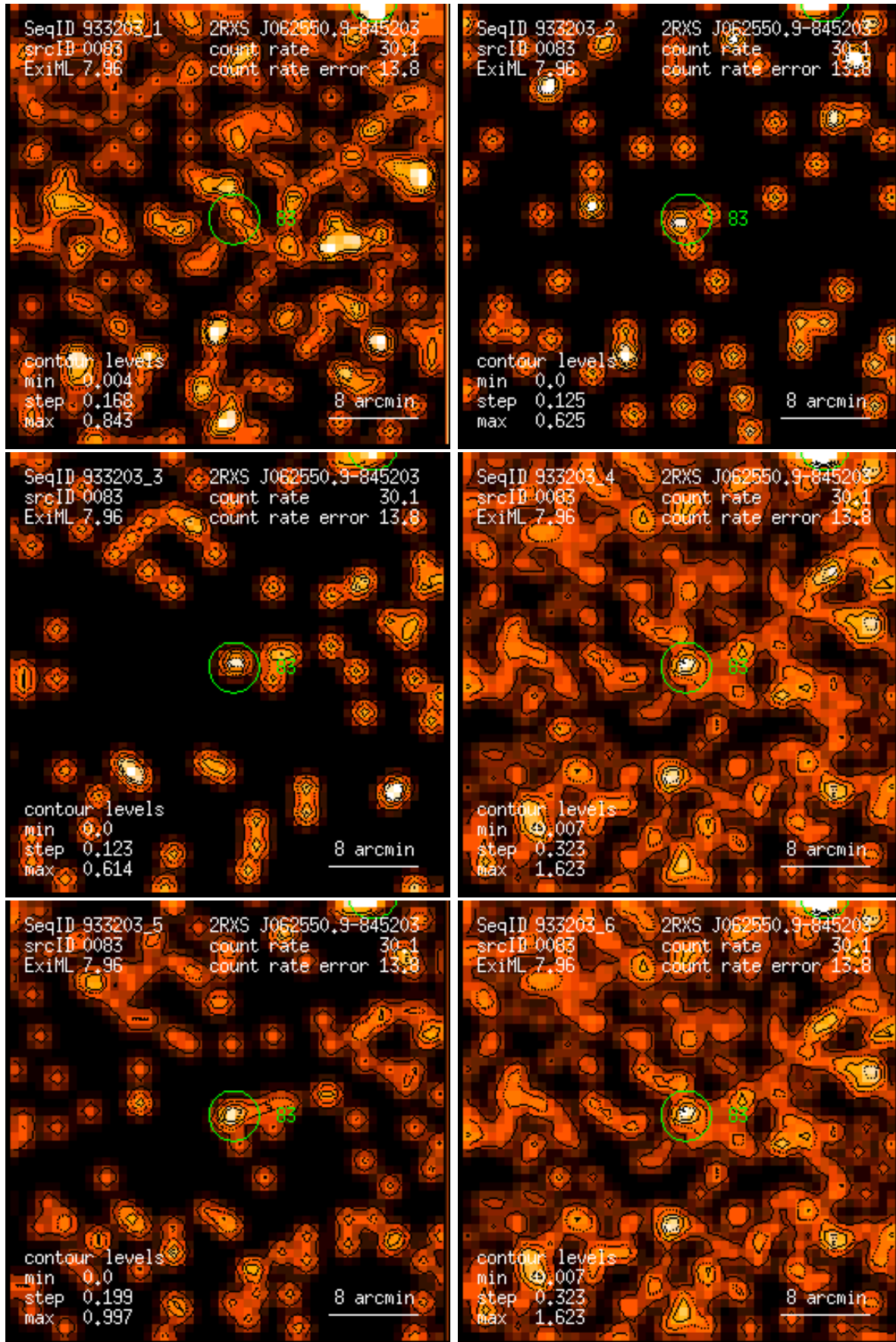
Figure 83: RASS 933203: detection 0083: band rate images, Gaussian filter: (1) PSPC channels 11 – 41, (2) 52 – 90, (3) 91 – 201, (4) 11 – 235, (5) 52 – 201, (6) 11 – 201. Broad band rates in counts/ks. Band rate contour levels in counts/ks/arcmin 2 .
