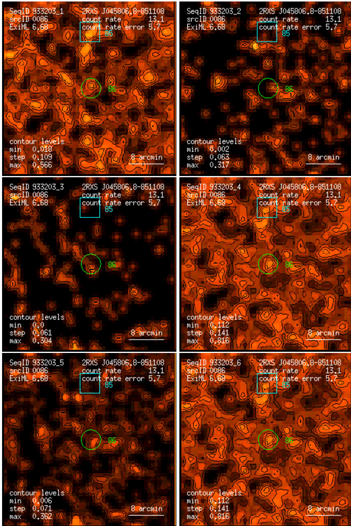
Figure 86: RASS 933203: detection 0086: band rate images, Gaussian filter: (1) PSPC channels 11 – 41, (2) 52 – 90, (3) 91 – 201, (4) 11 – 235, (5) 52 – 201, (6) 11 – 201. Broad band rates in counts/ks. Band rate contour levels in counts/ks/arcmin 2 .
