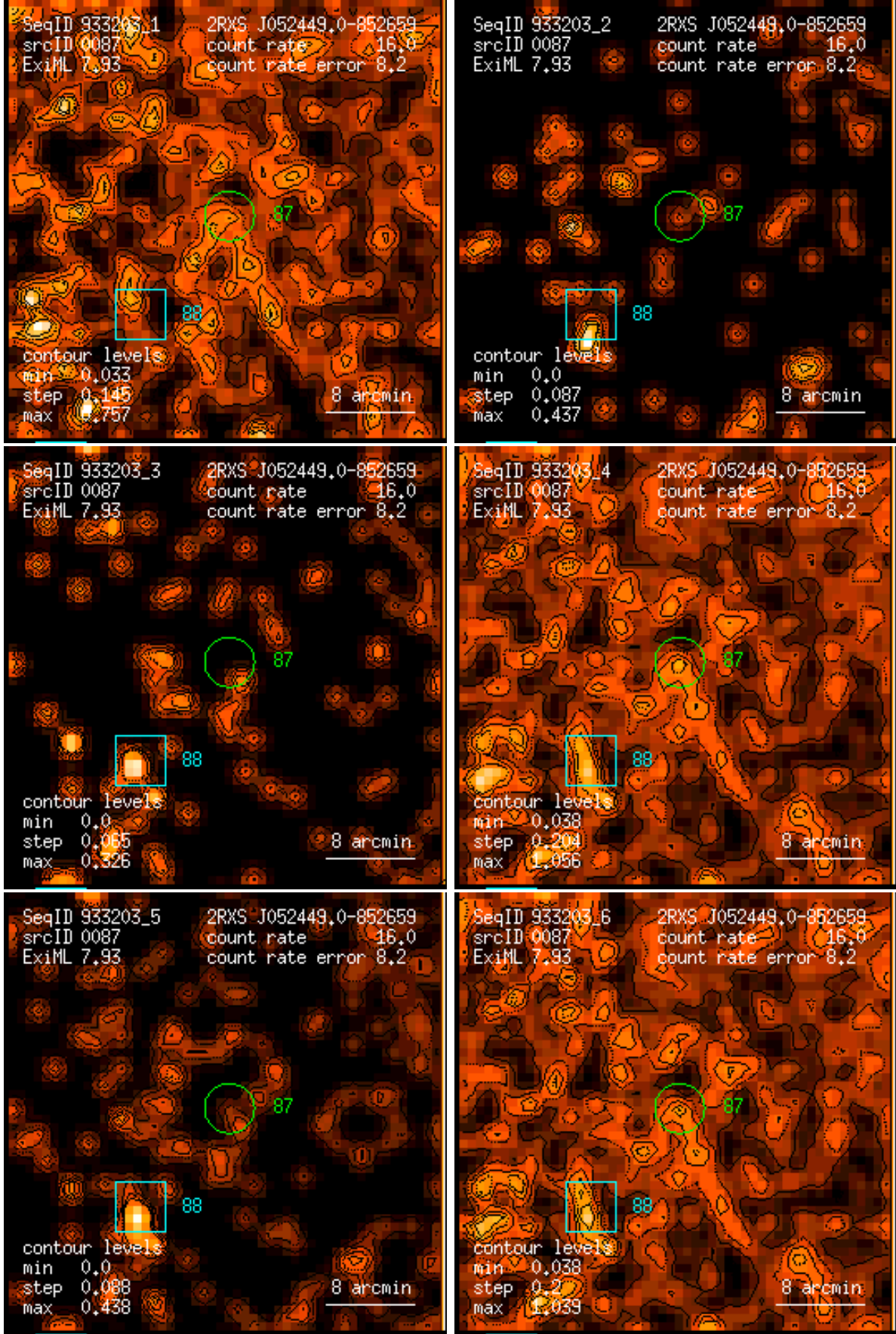
Figure 87: RASS 933203: detection 0087: band rate images, Gaussian filter: (1) PSPC channels 11 – 41, (2) 52 – 90, (3) 91 – 201, (4) 11 – 235, (5) 52 – 201, (6) 11 – 201. Broad band rates in counts/ks. Band rate contour levels in counts/ks/arcmin 2 .
