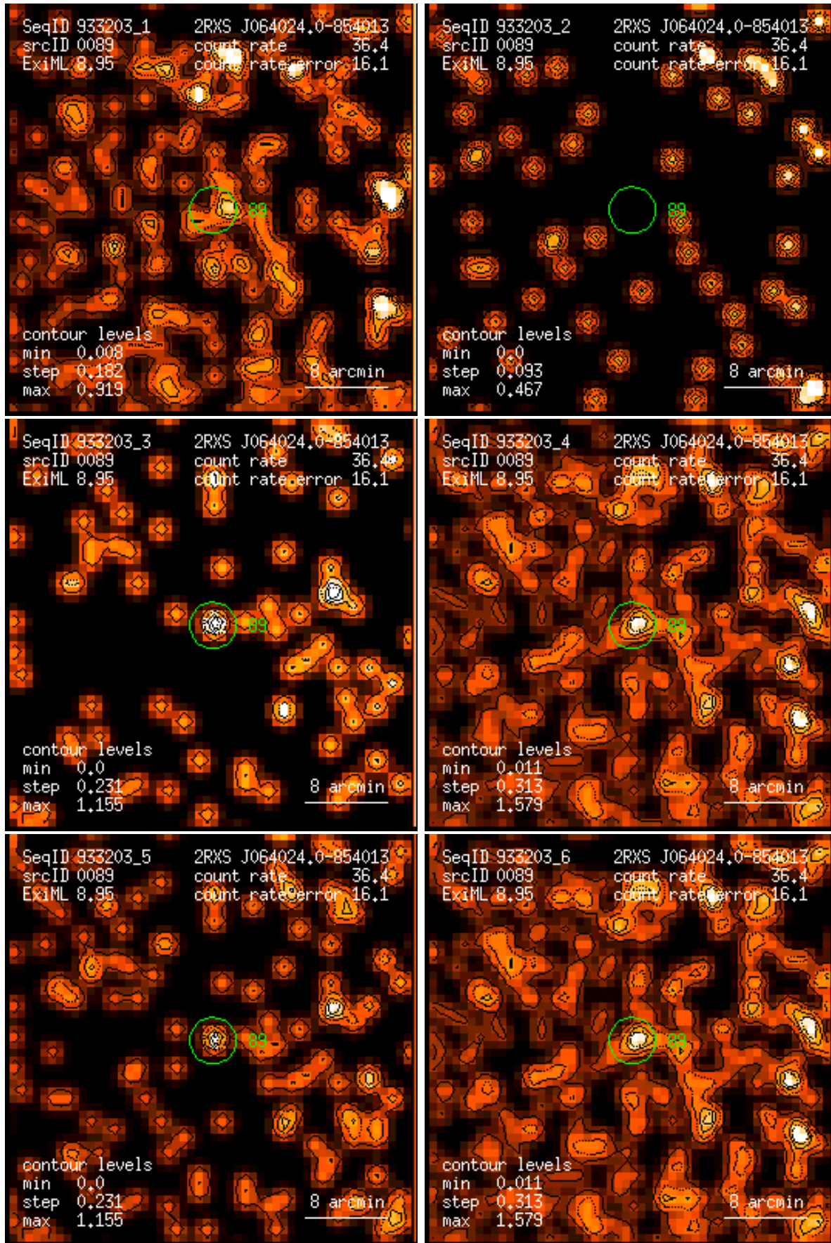
Figure 89: RASS 933203: detection 0089: band rate images, Gaussian filter: (1) PSPC channels 11 – 41, (2) 52 – 90, (3) 91 – 201, (4) 11 – 235, (5) 52 – 201, (6) 11 – 201. Broad band rates in counts/ks. Band rate contour levels in counts/ks/arcmin 2 .
