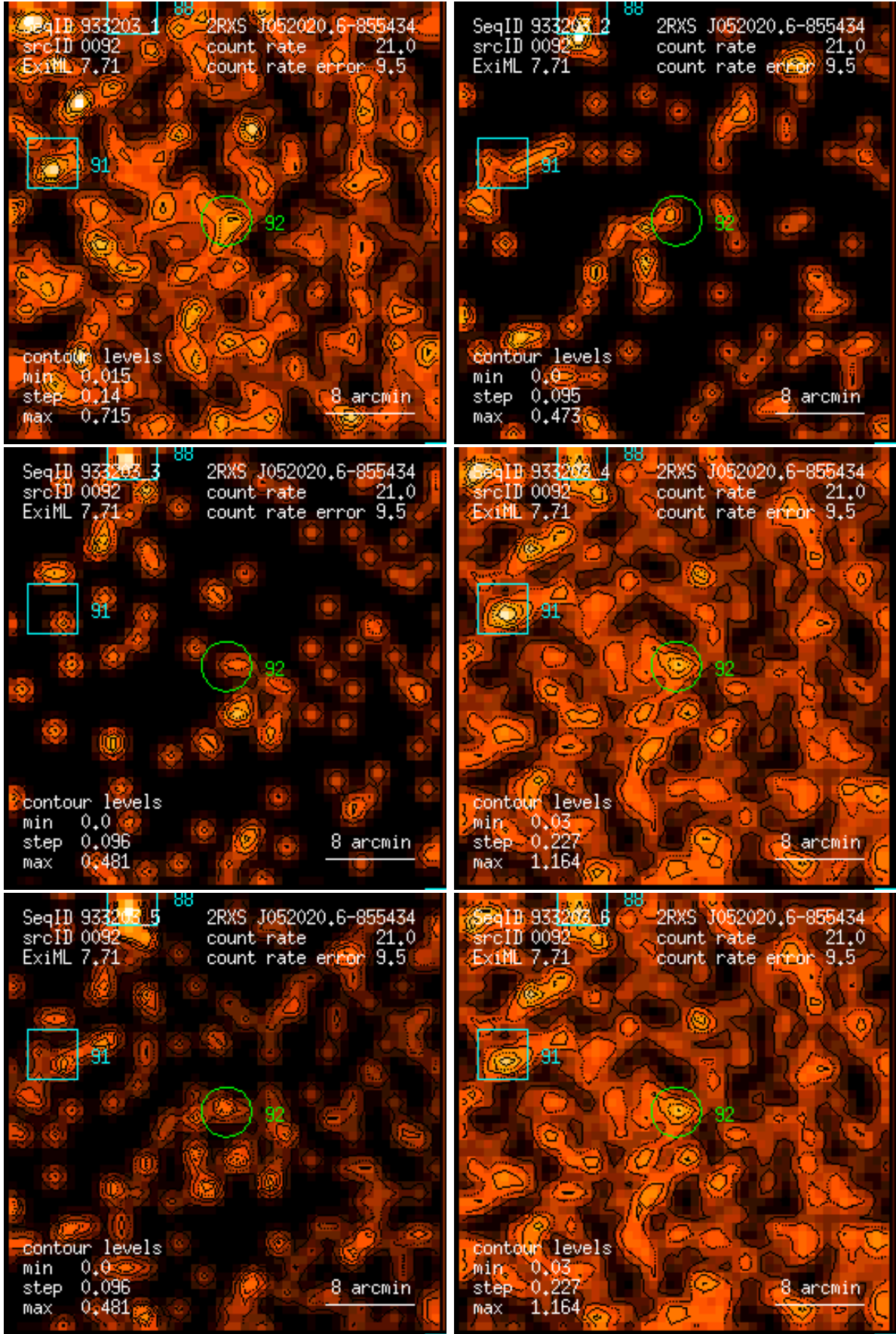
Figure 92: RASS 933203: detection 0092: band rate images, Gaussian filter: (1) PSPC channels 11 – 41, (2) 52 – 90, (3) 91 – 201, (4) 11 – 235, (5) 52 – 201, (6) 11 – 201. Broad band rates in counts/ks. Band rate contour levels in counts/ks/arcmin 2 .
