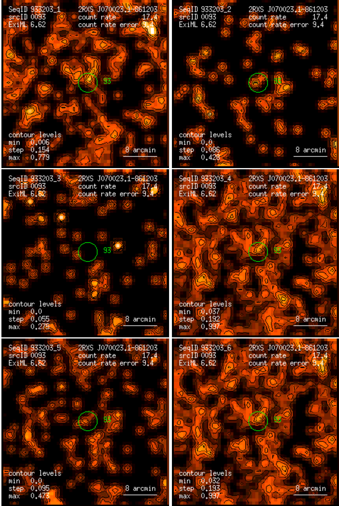
Figure 93: RASS 933203: detection 0093: band rate images, Gaussian filter: (1) PSPC channels 11 – 41, (2) 52 – 90, (3) 91 – 201, (4) 11 – 235, (5) 52 – 201, (6) 11 – 201. Broad band rates in counts/ks. Band rate contour levels in counts/ks/arcmin 2 .
