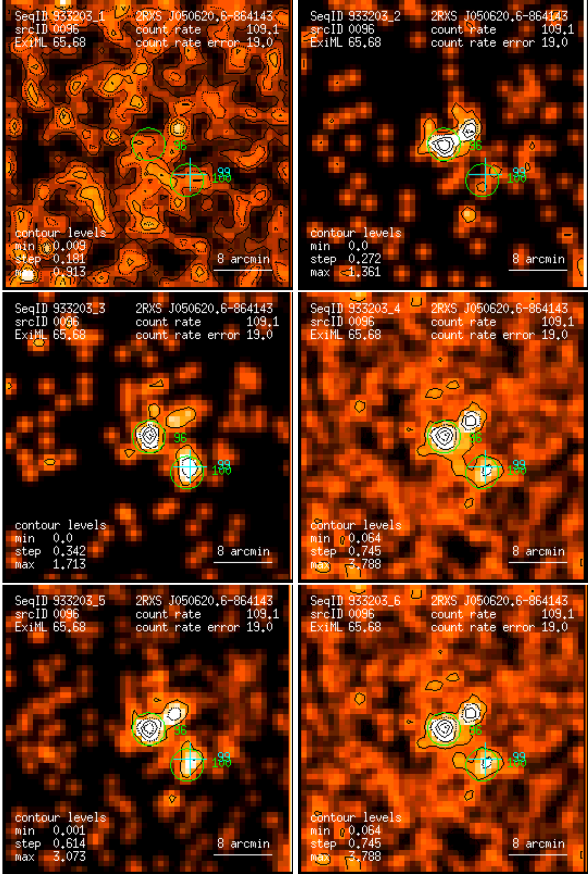
Figure 96: RASS 933203: detection 0096: band rate images, Gaussian filter: (1) PSPC channels 11 – 41, (2) 52 – 90, (3) 91 – 201, (4) 11 – 235, (5) 52 – 201, (6) 11 – 201. Broad band rates in counts/ks. Band rate contour levels in counts/ks/arcmin 2 .
