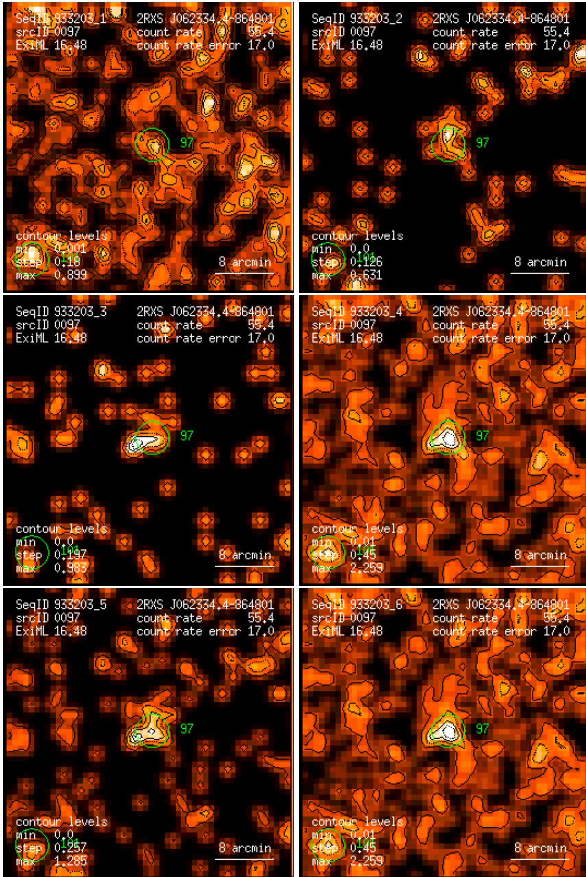
Figure 97: RASS 933203: detection 0097: band rate images, Gaussian filter: (1) PSPC channels 11 – 41, (2) 52 – 90, (3) 91 – 201, (4) 11 – 235, (5) 52 – 201, (6) 11 – 201. Broad band rates in counts/ks. Band rate contour levels in counts/ks/arcmin 2 .
