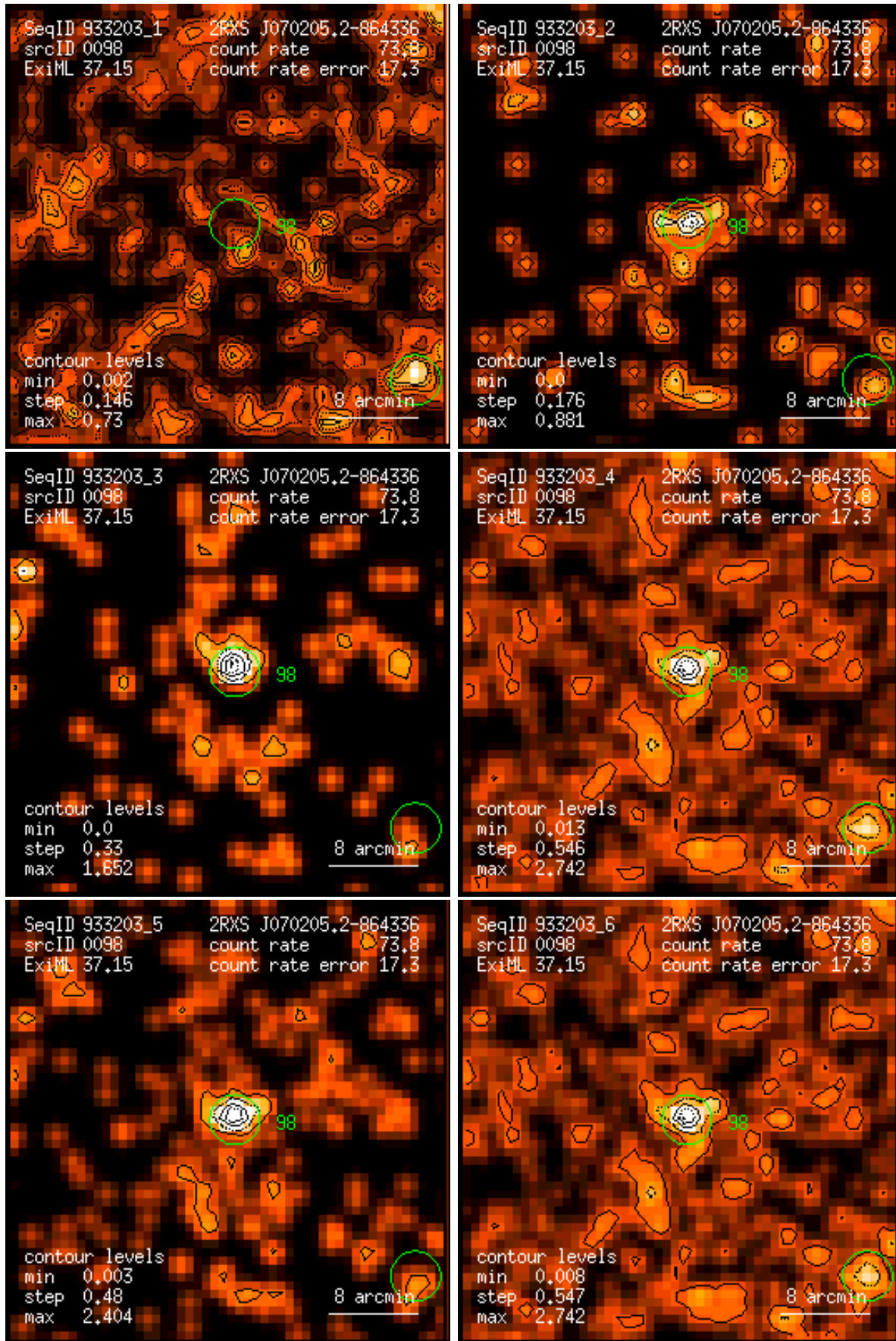
Figure 98: RASS 933203: detection 0098: band rate images, Gaussian filter: (1) PSPC channels 11 – 41, (2) 52 – 90, (3) 91 – 201, (4) 11 – 235, (5) 52 – 201, (6) 11 – 201. Broad band rates in counts/ks. Band rate contour levels in counts/ks/arcmin 2 .
