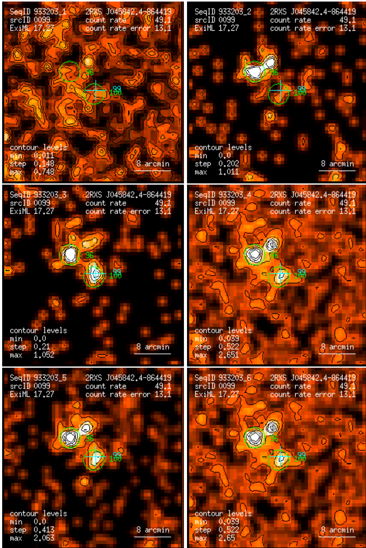
Figure 99: RASS 933203: detection 0099: band rate images, Gaussian filter: (1) PSPC channels 11 – 41, (2) 52 – 90, (3) 91 – 201, (4) 11 – 235, (5) 52 – 201, (6) 11 – 201. Broad band rates in counts/ks. Band rate contour levels in counts/ks/arcmin 2 .
