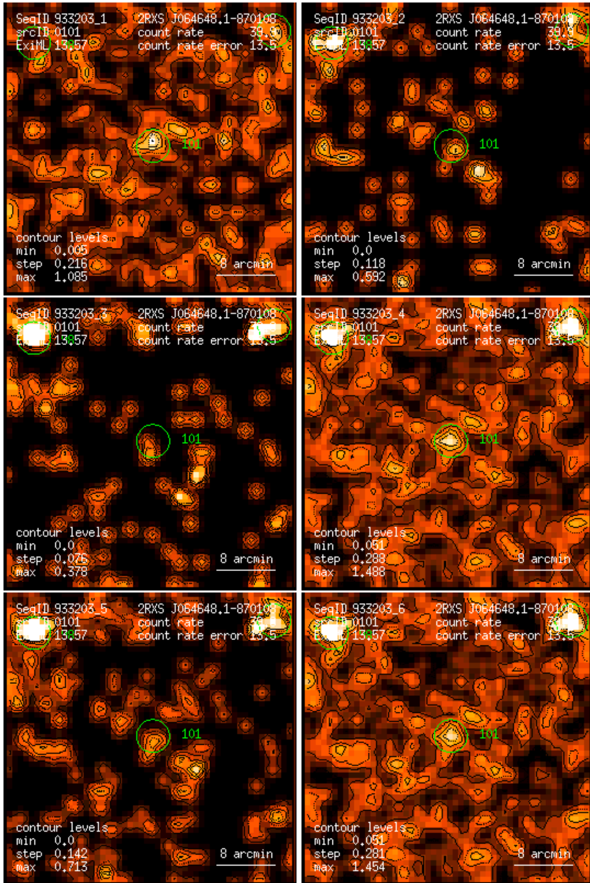
Figure 101: RASS 933203: detection 0101: band rate images, Gaussian filter: (1) PSPC channels 11 – 41, (2) 52 – 90, (3) 91 – 201, (4) 11 – 235, (5) 52 – 201, (6) 11 – 201. Broad band rates in counts/ks. Band rate contour levels in counts/ks/arcmin 2 .
