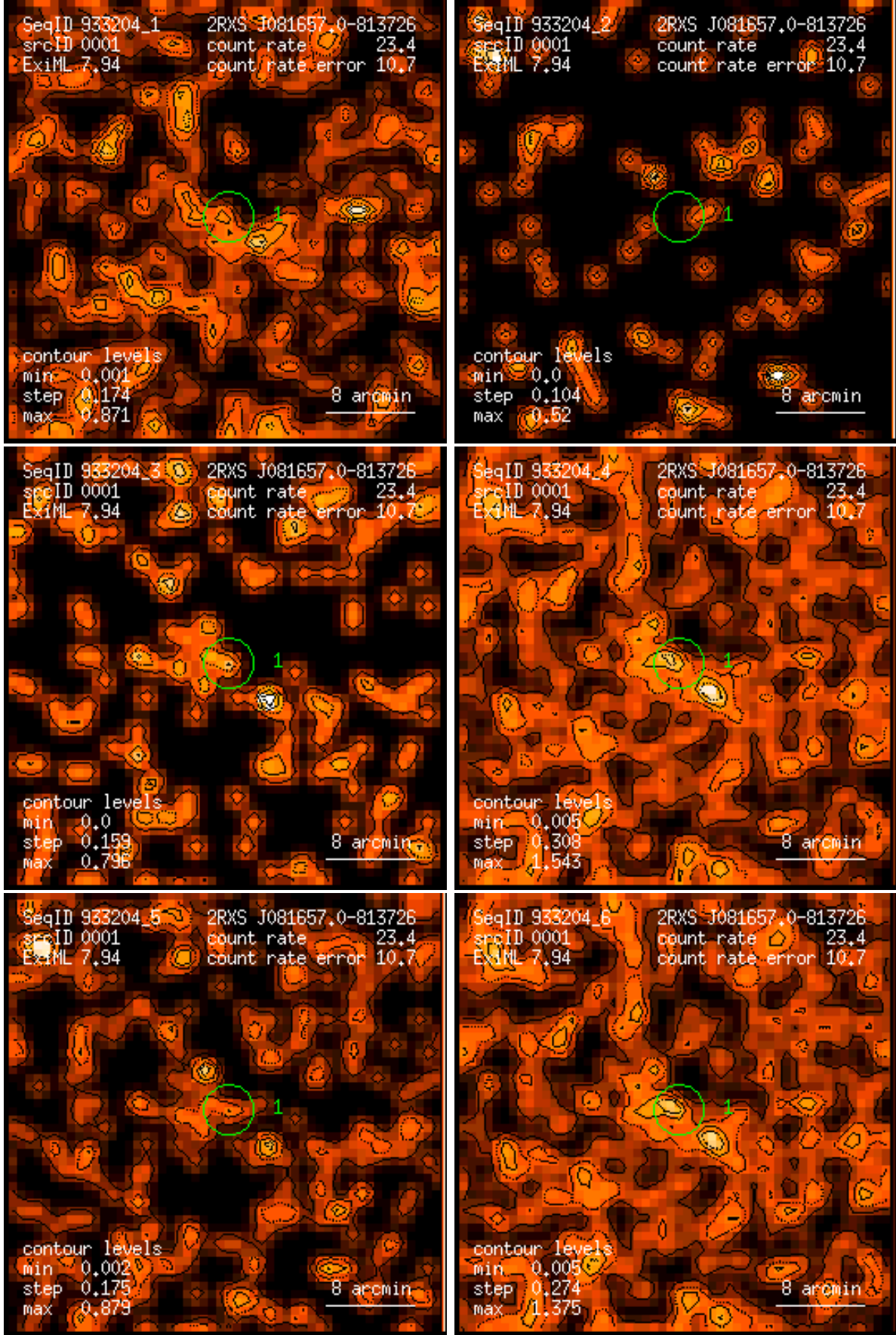
Figure 1: RASS 933204: detection 0001: band rate images, Gaussian filter: (1) PSPC channels 11 – 41, (2) 52 – 90, (3) 91 – 201, (4) 11 – 235, (5) 52 – 201, (6) 11 – 201. Broad band rates in counts/ks. Band rate contour levels in counts/ks/arcmin 2 .
