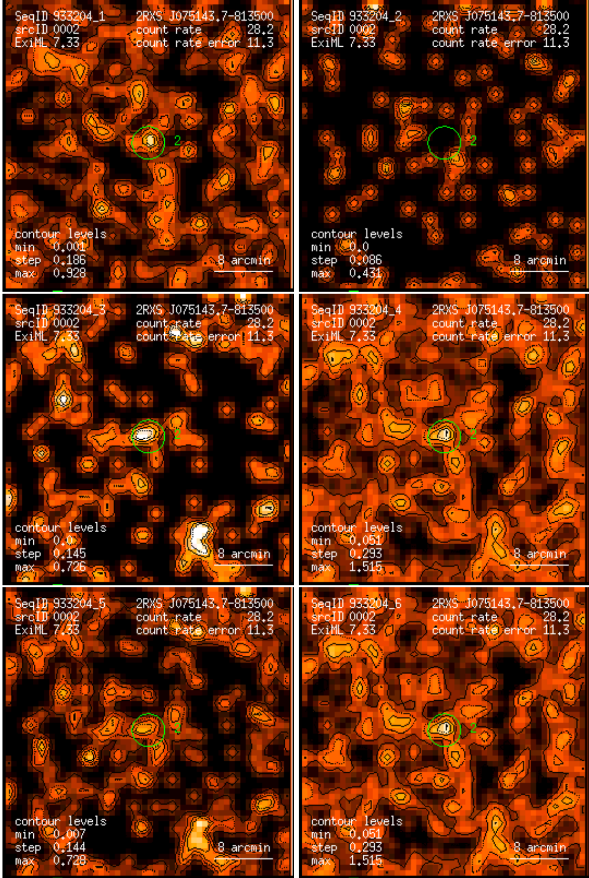
Figure 2: RASS 933204: detection 0002: band rate images, Gaussian filter: (1) PSPC channels 11 – 41, (2) 52 – 90, (3) 91 – 201, (4) 11 – 235, (5) 52 – 201, (6) 11 – 201. Broad band rates in counts/ks. Band rate contour levels in counts/ks/arcmin 2 .
