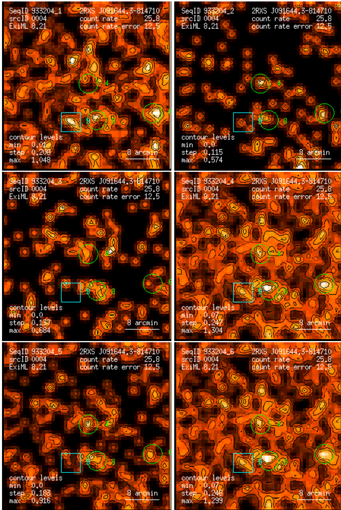
Figure 4: RASS 933204: detection 0004: band rate images, Gaussian filter: (1) PSPC channels 11 – 41, (2) 52 – 90, (3) 91 – 201, (4) 11 – 235, (5) 52 – 201, (6) 11 – 201. Broad band rates in counts/ks. Band rate contour levels in counts/ks/arcmin 2 .
