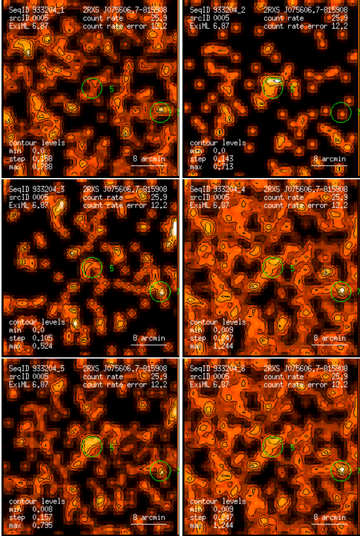
Figure 5: RASS 933204: detection 0005: band rate images, Gaussian filter: (1) PSPC channels 11 – 41, (2) 52 – 90, (3) 91 – 201, (4) 11 – 235, (5) 52 – 201, (6) 11 – 201. Broad band rates in counts/ks. Band rate contour levels in counts/ks/arcmin 2 .
